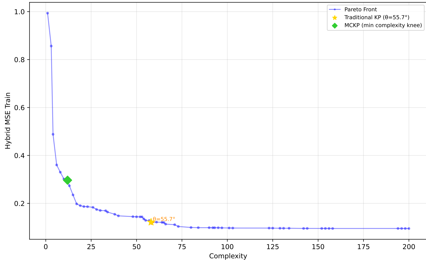
589_fri_c2_1000_25 - Run 6 - SVP - Hybrid MSE Train \lambda_1=0.20 , \lambda_2=0.00 , \lambda_3=1.00 | Difficulty: 1.00 | Method: hmr
