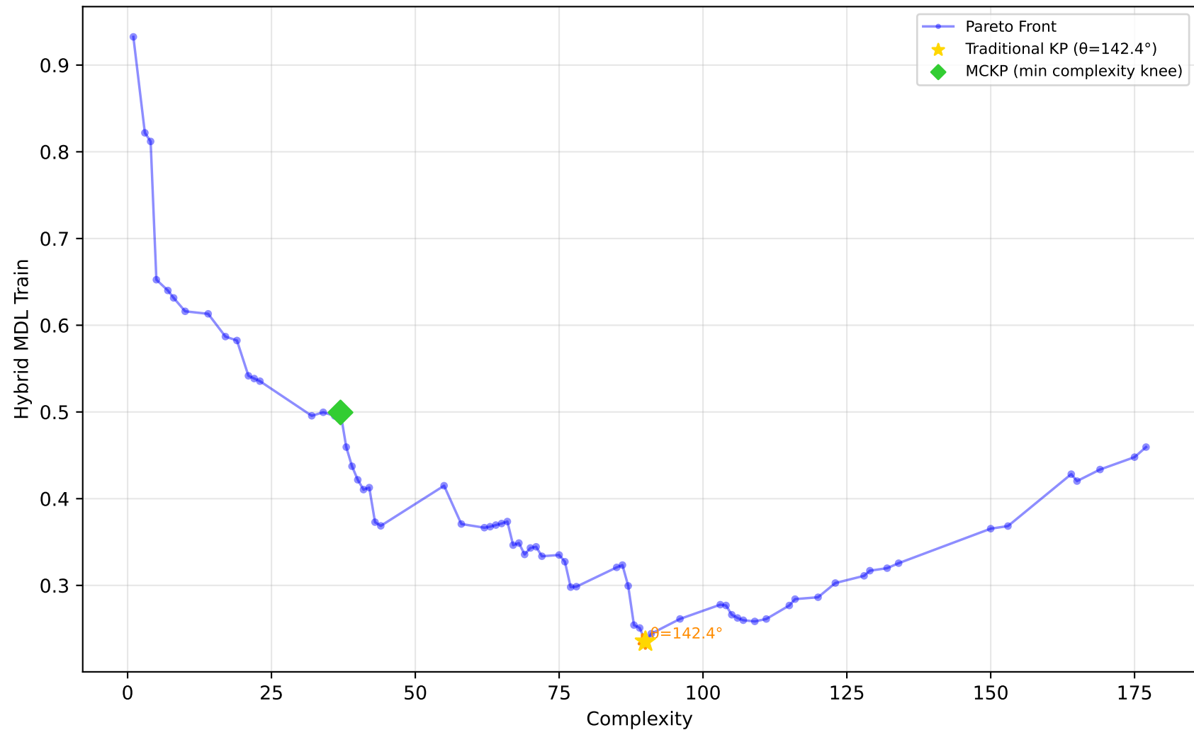
589_fri_c2_1000_25 - Run 7 - MVP - Hybrid MDL Train \lambda_1=0.00, \bar{\lambda}_2=0.00, \bar{\lambda}_3=0.00 | Difficulty: 1.00 | Method: hmr
