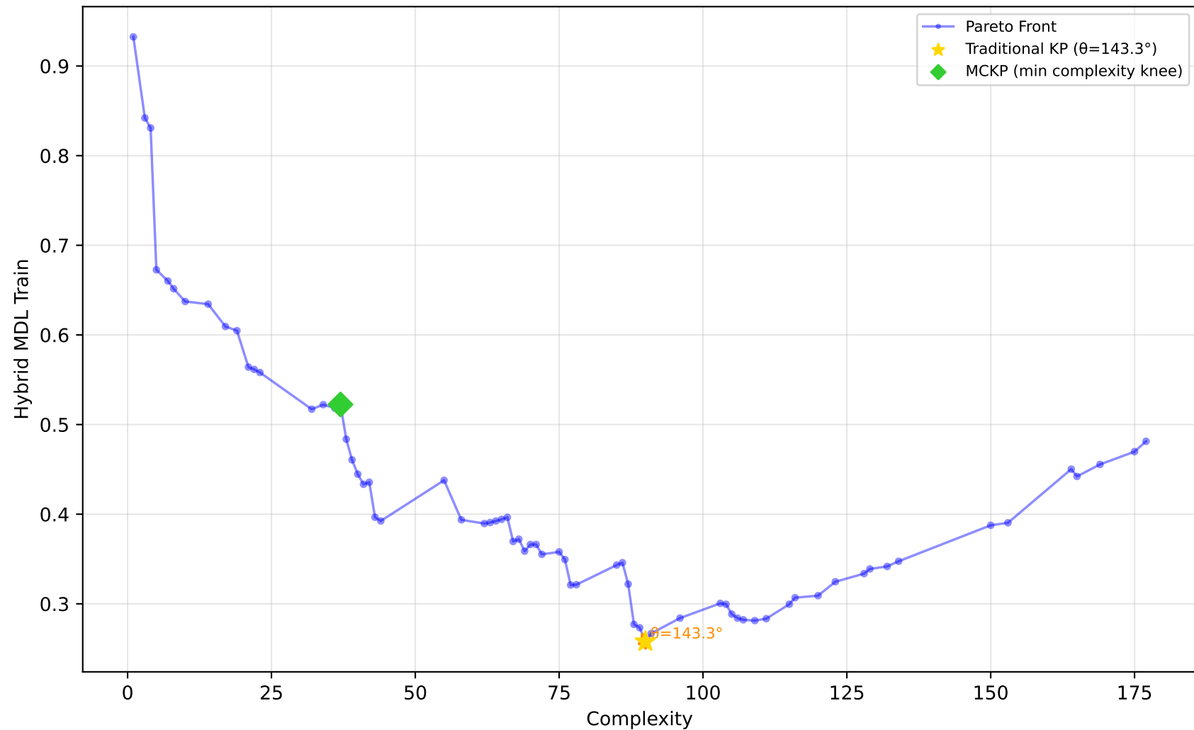
589_fri_c2_1000_25 - Run 7 - MVP - Hybrid MDL Train \lambda_1=0.30, \bar{\lambda}_2=0.00, \bar{\lambda}_3=0.20 | Difficulty: 1.00 | Method: hmr
