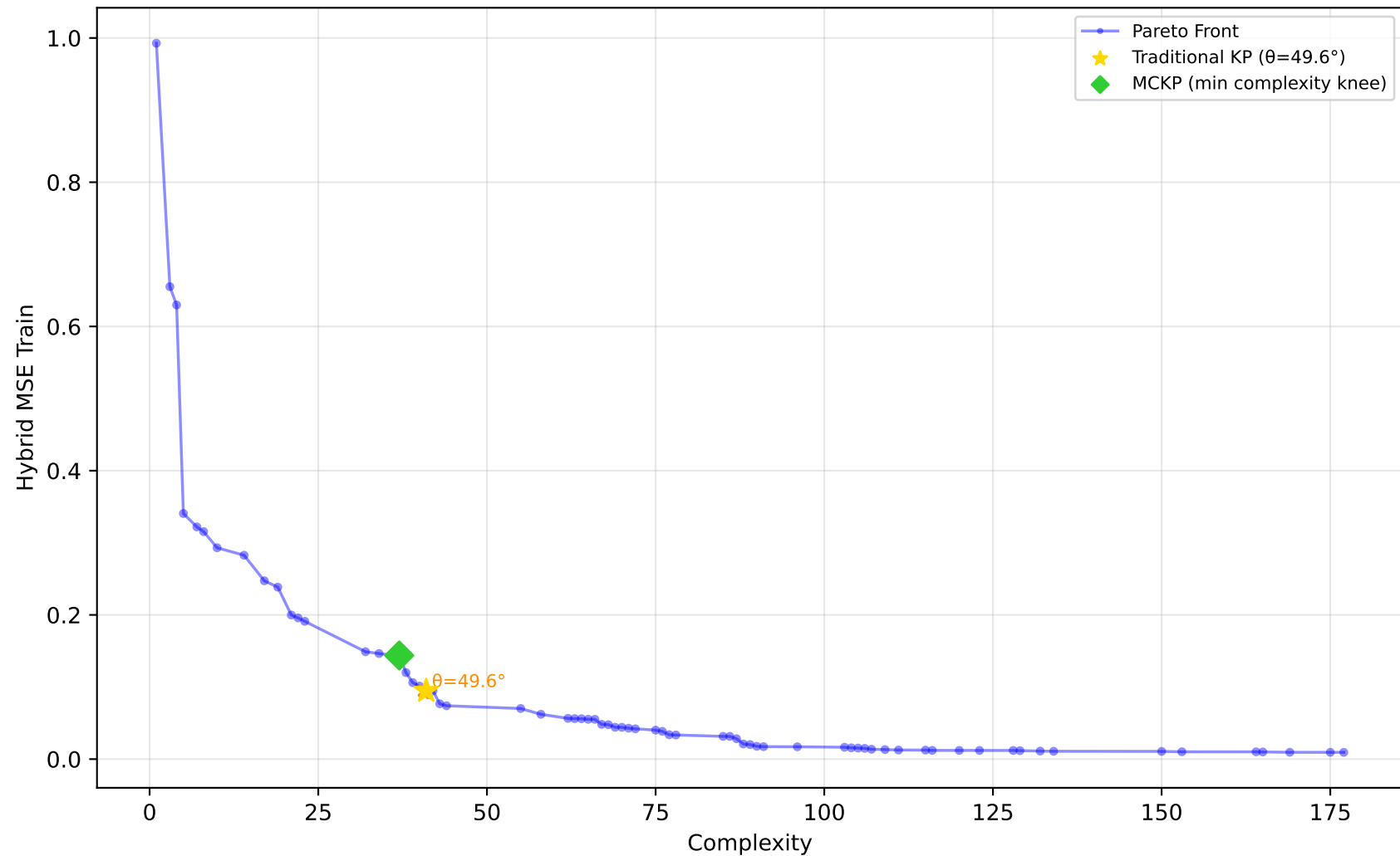
589_fri_c2_1000_25 - Run 7 - MVP - Hybrid MSE Train \lambda_1=0.00, \bar{\lambda}_2=0.00, \bar{\lambda}_3=0.00 | Difficulty: 1.00 | Method: hmr
