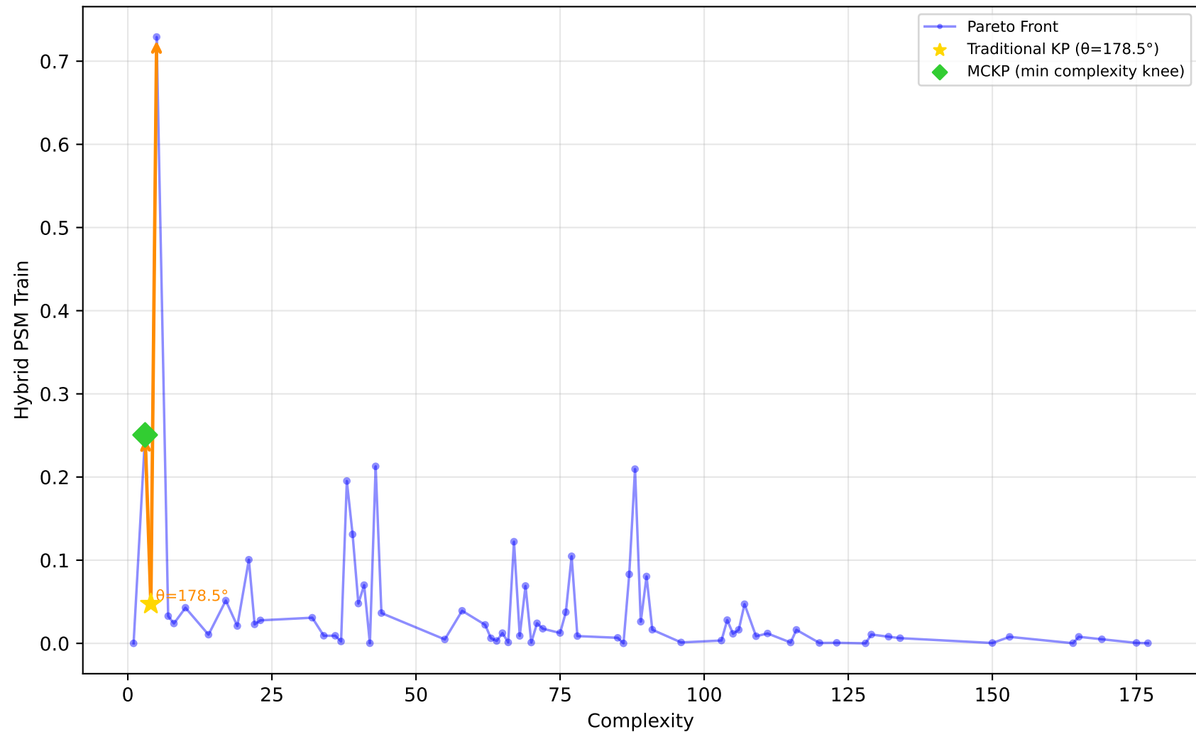
589_fri_c2_1000_25 - Run 7 - MVP - Hybrid PSM Train \lambda_1=0.00, \bar{\lambda}_2=0.00, \bar{\lambda}_3=0.00 | Difficulty: 1.00 | Method: hmr
