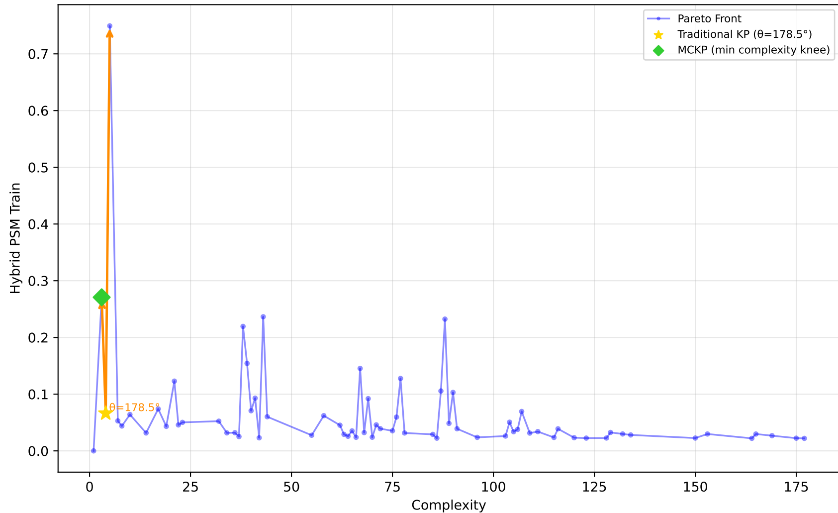
589_fri_c2_1000_25 - Run 7 - MVP - Hybrid PSM Train \lambda_1=0.30, \bar{\lambda}_2=0.00, \bar{\lambda}_3=0.20 | Difficulty: 1.00 | Method: hmr
