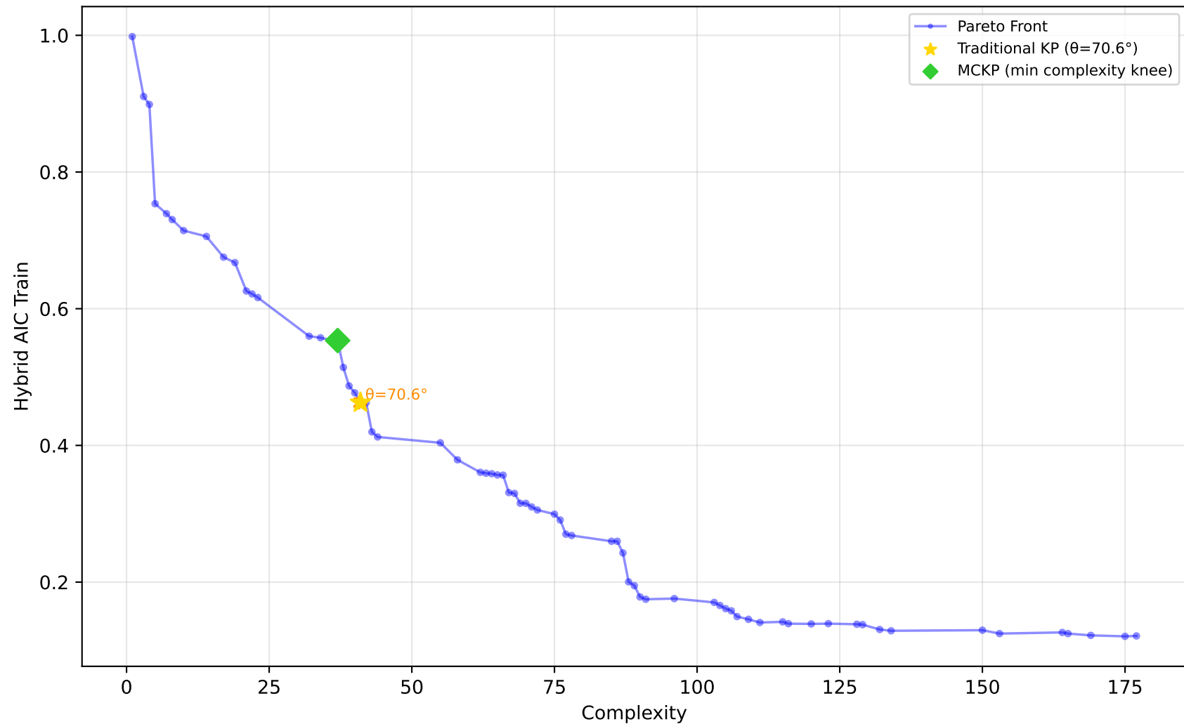
589_fri_c2_1000_25 - Run 7 - SVP - Hybrid AIC Train \lambda_1=0.20 , \lambda_2=0.00 , \lambda_3=1.00 | Difficulty: 1.00 | Method: hmr
