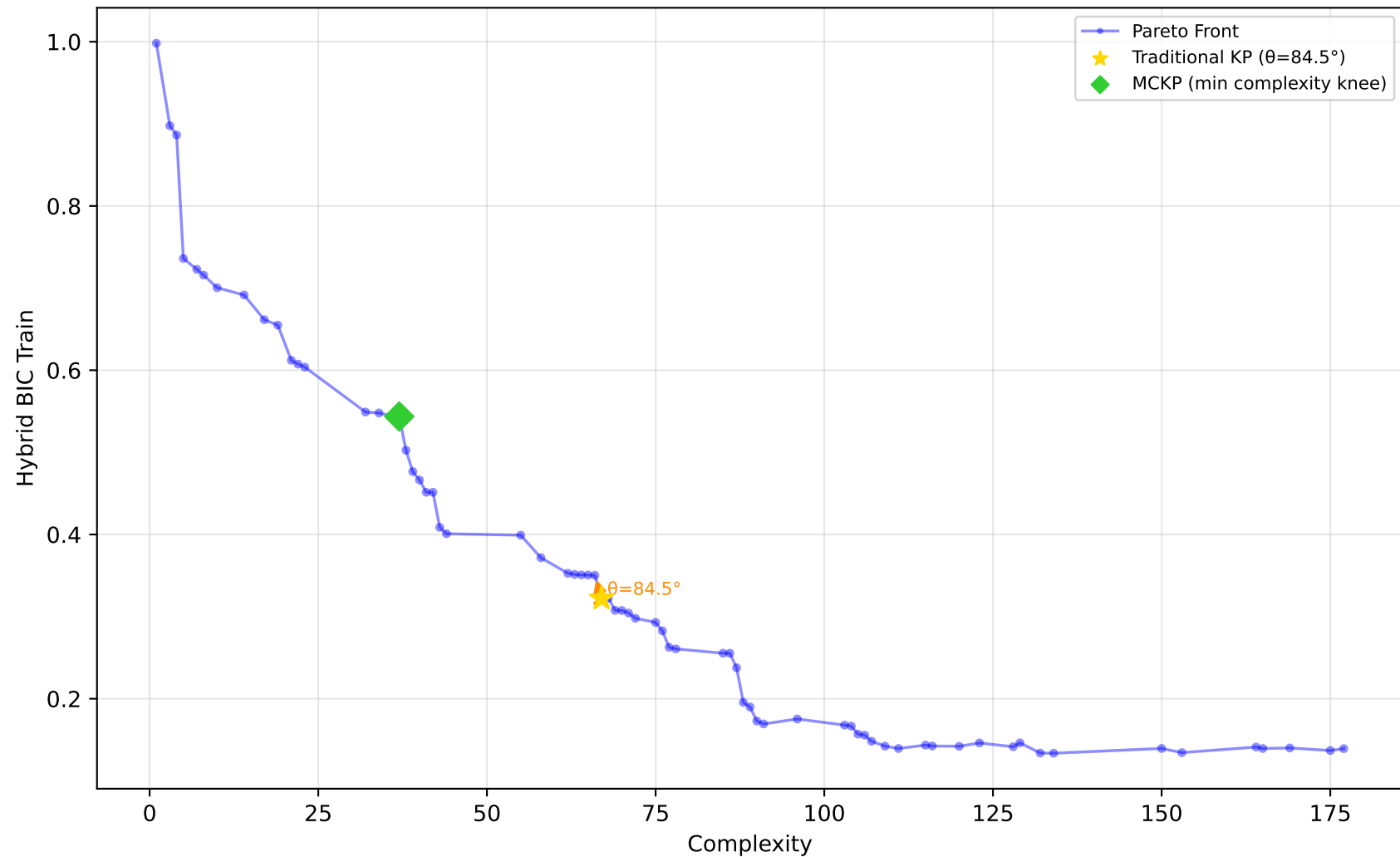
589_fri_c2_1000_25 - Run 7 - SVP - Hybrid BIC Train \lambda_1=0.10, \lambda_2=0.00, \lambda_3=0.10 | Difficulty: 1.00 | Method: hmr
