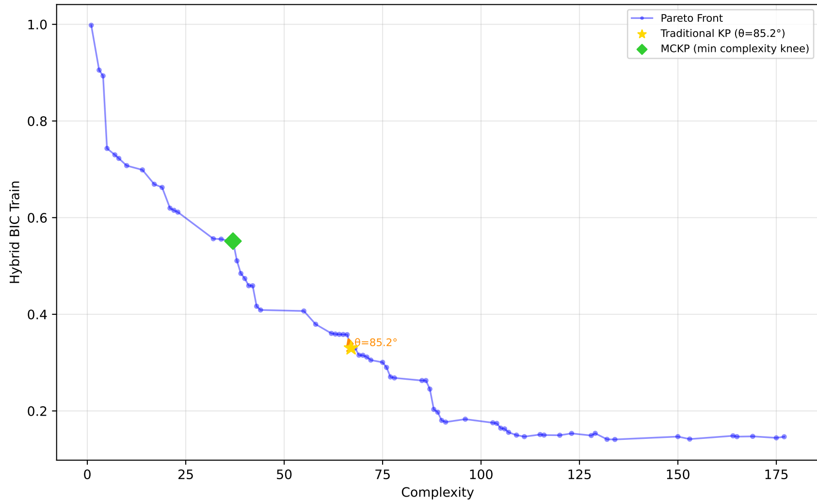
589_fri_c2_1000_25 - Run 7 - SVP - Hybrid BIC Train \lambda_1=0.20, \lambda_2=0.00, \lambda_3=1.00 | Difficulty: 1.00 | Method: hmr
