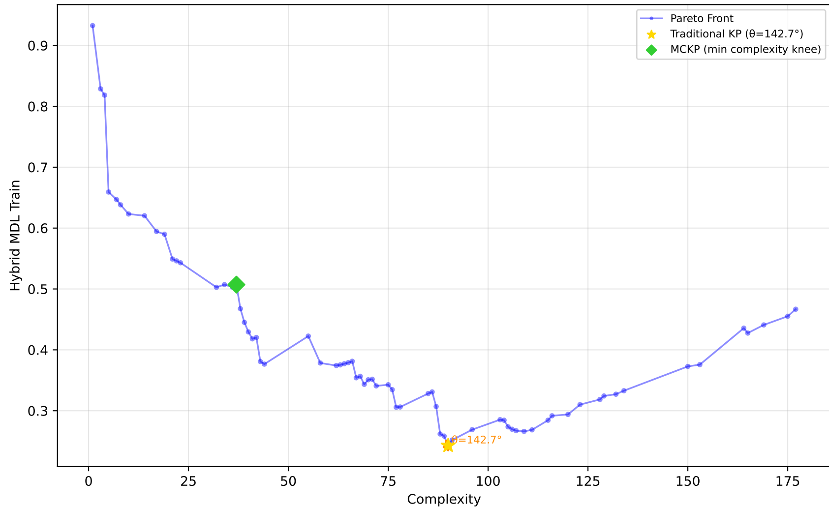
589_fri_c2_1000_25 - Run 7 - SVP - Hybrid MDL Train \lambda_1=0.10, \lambda_2=0.00, \lambda_3=0.10 | Difficulty: 1.00 | Method: hmr
