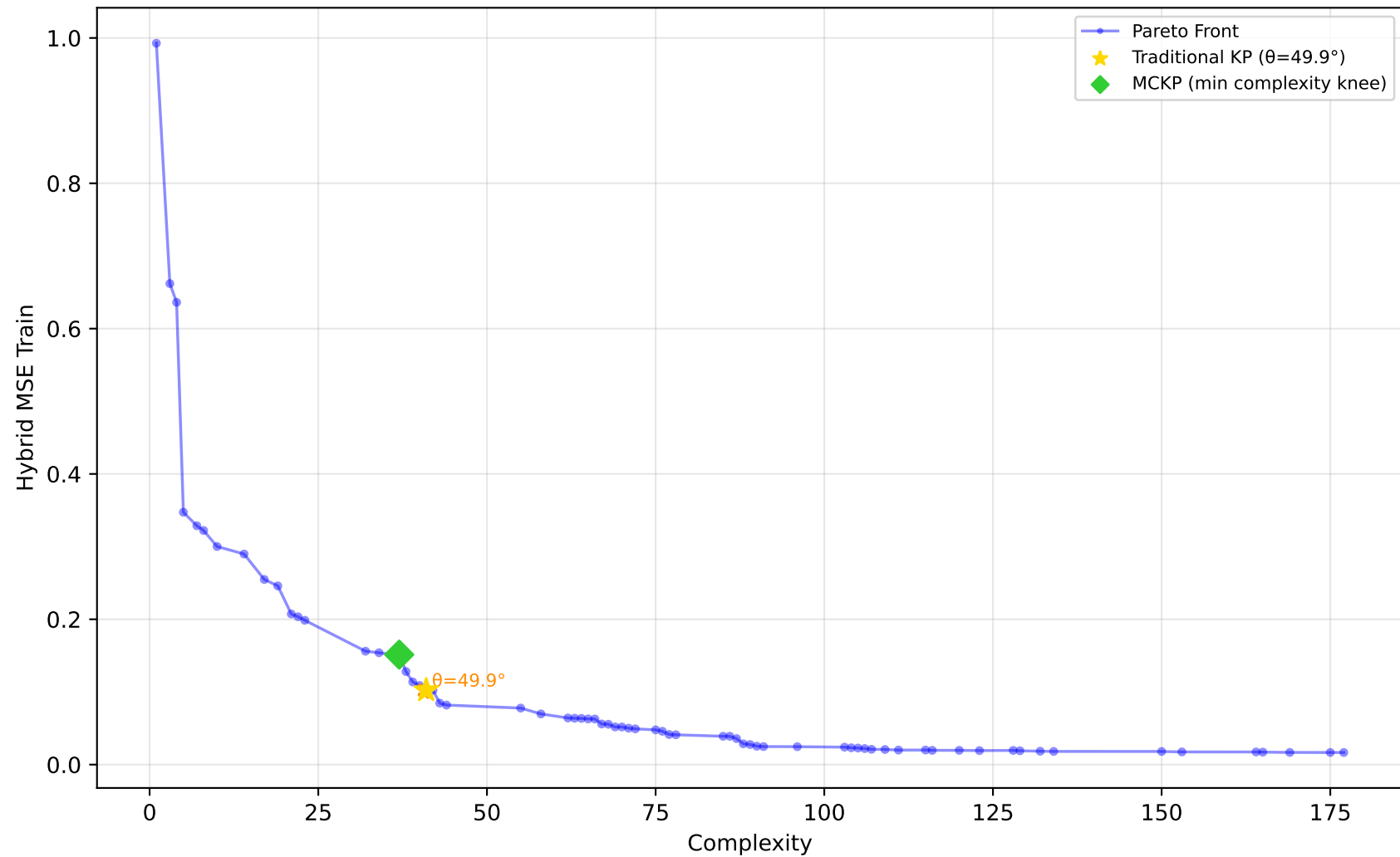
589_fri_c2_1000_25 - Run 7 - SVP - Hybrid MSE Train \lambda_1=0.10, \lambda_2=0.00, \lambda_3=0.10 | Difficulty: 1.00 | Method: hmr
