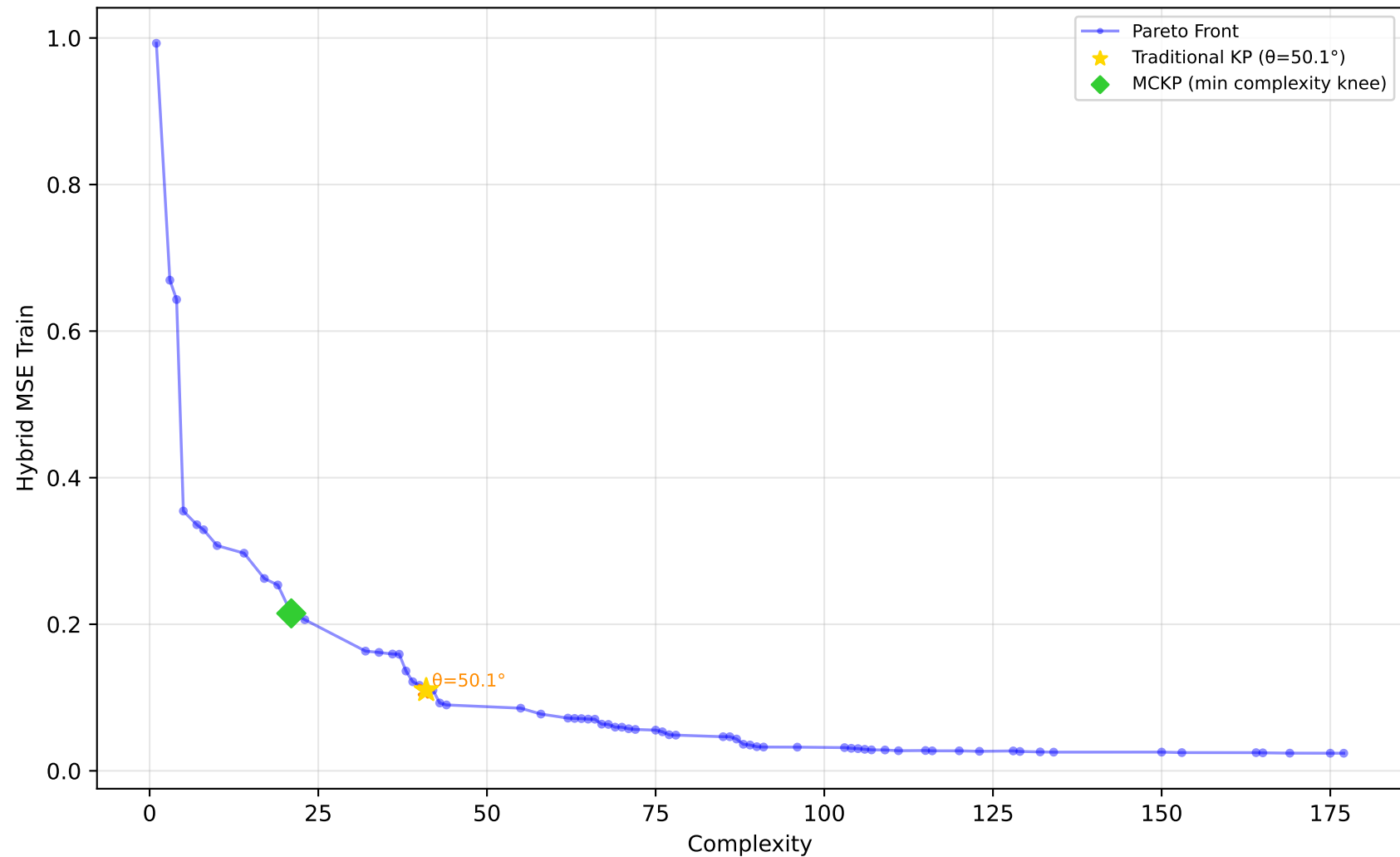
589_fri_c2_1000_25 - Run 7 - SVP - Hybrid MSE Train \lambda_1=0.20 , \lambda_2=0.00 , \lambda_3=1.00 | Difficulty: 1.00 | Method: hmr
