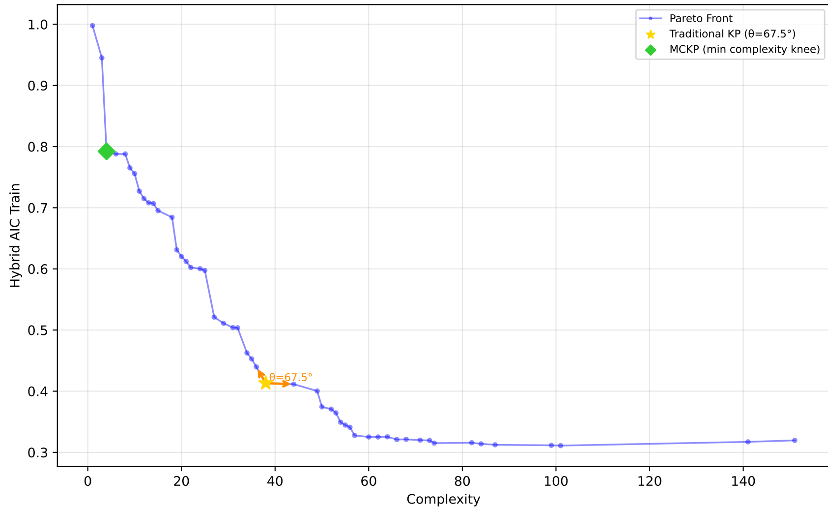
589_fri_c2_1000_25 - Run 8 - MVP - Hybrid AIC Train \lambda_1=0.00, \lambda_2=0.00, \lambda_3=0.00 | Difficulty: 1.00 | Method: hmr
