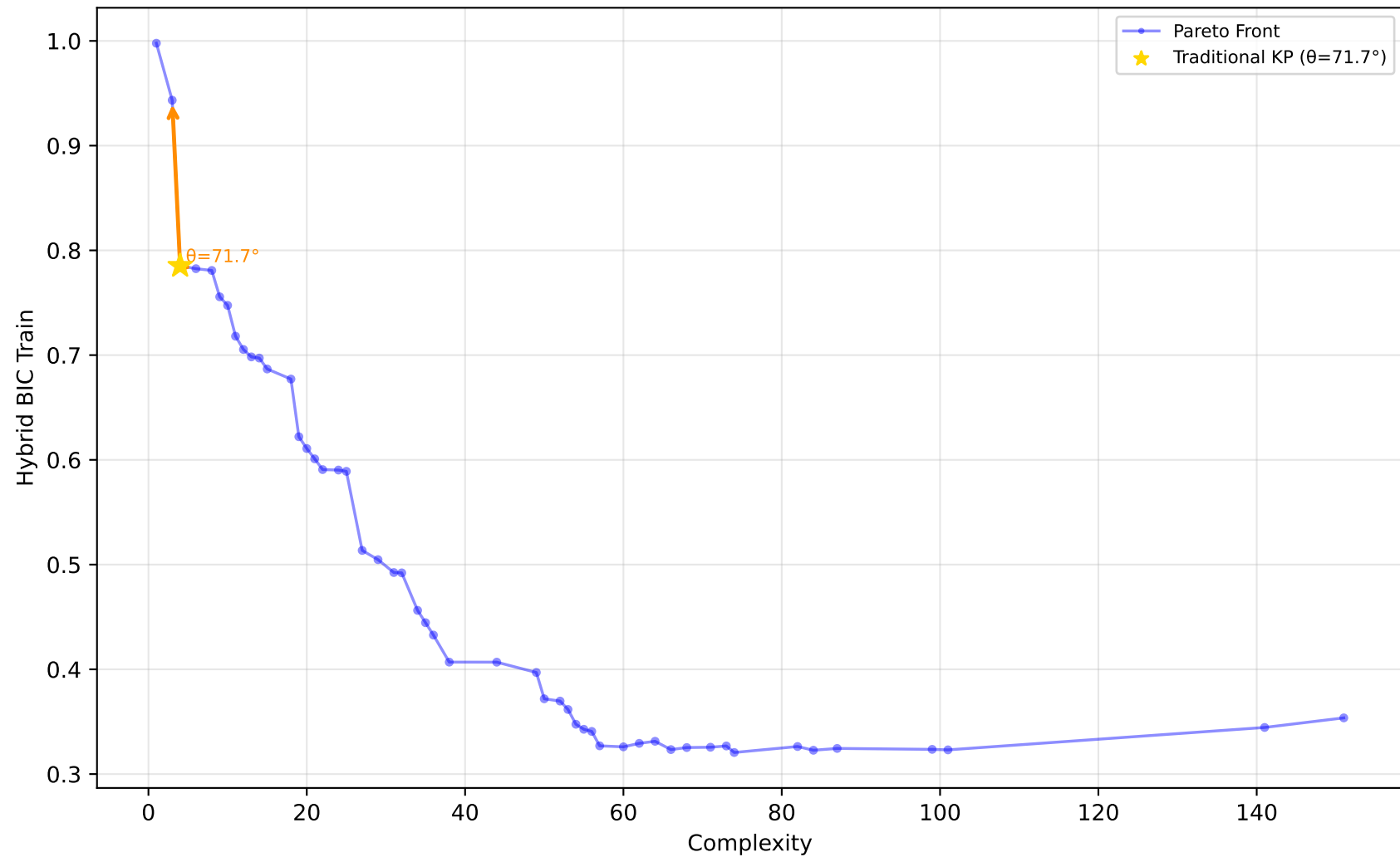
589_fri_c2_1000_25 - Run 8 - MVP - Hybrid BIC Train \lambda_1=0.00, \lambda_2=0.00, \lambda_3=0.00 | Difficulty: 1.00 | Method: hmr
