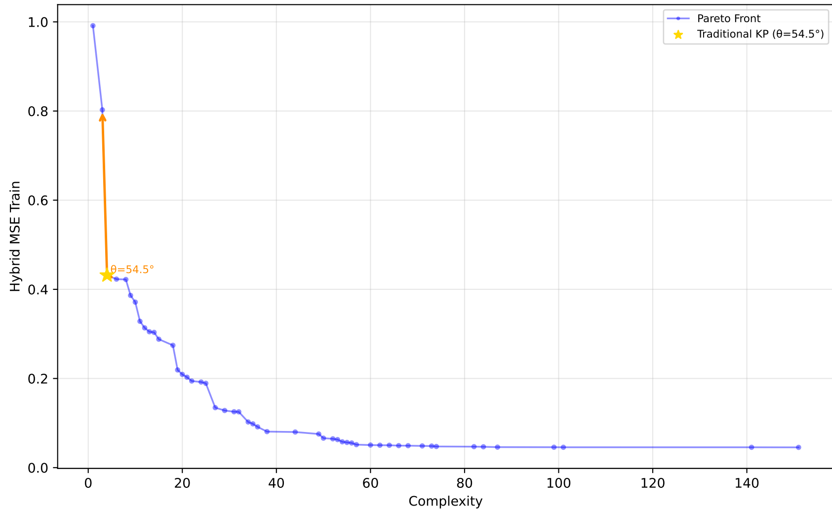
589_fri_c2_1000_25 - Run 8 - MVP - Hybrid MSE Train \lambda_1=0.00, \bar{\lambda}_2=0.00, \bar{\lambda}_3=0.00 | Difficulty: 1.00 | Method: hmr
