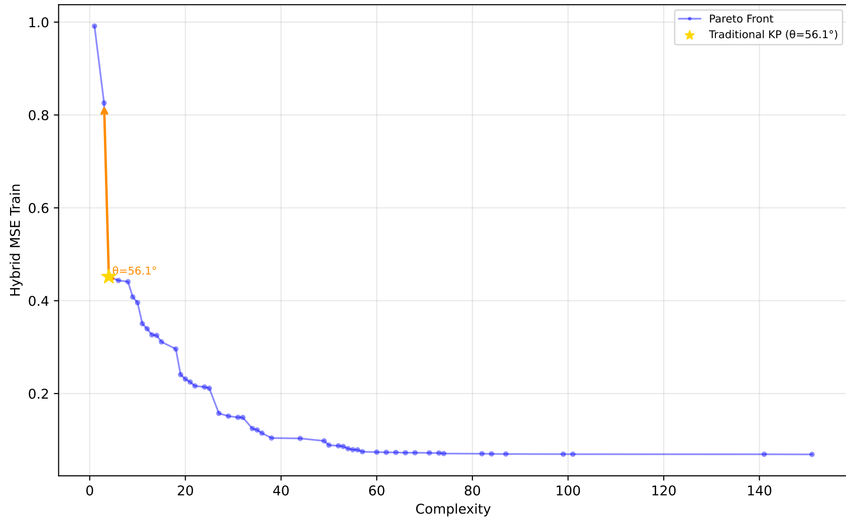
589_fri_c2_1000_25 - Run 8 - MVP - Hybrid MSE Train \lambda_1=0.30, \bar{\lambda}_2=0.00, \bar{\lambda}_3=0.20 | Difficulty: 1.00 | Method: hmr
