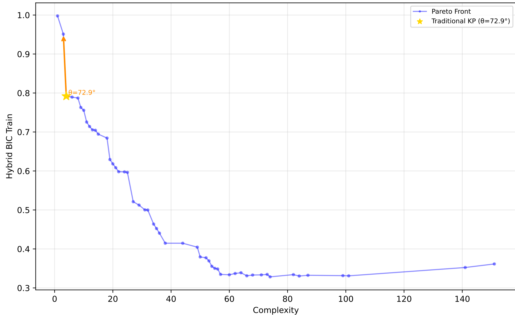
589_fri_c2_1000_25 - Run 8 - SVP - Hybrid BIC Train \lambda_1=0.10, \lambda_2=0.00, \lambda_3=0.10 | Difficulty: 1.00 | Method: hmr
