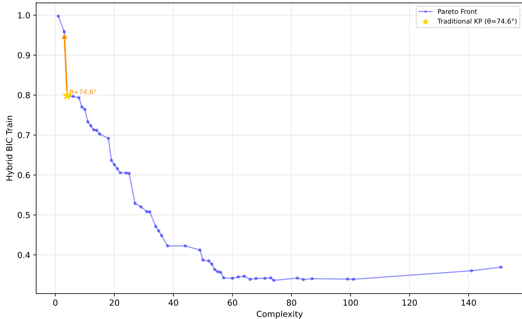
589_fri_c2_1000_25 - Run 8 - SVP - Hybrid BIC Train \lambda_1=0.20 , \lambda_2=0.00 , \lambda_3=1.00 | Difficulty: 1.00 | Method: hmr
