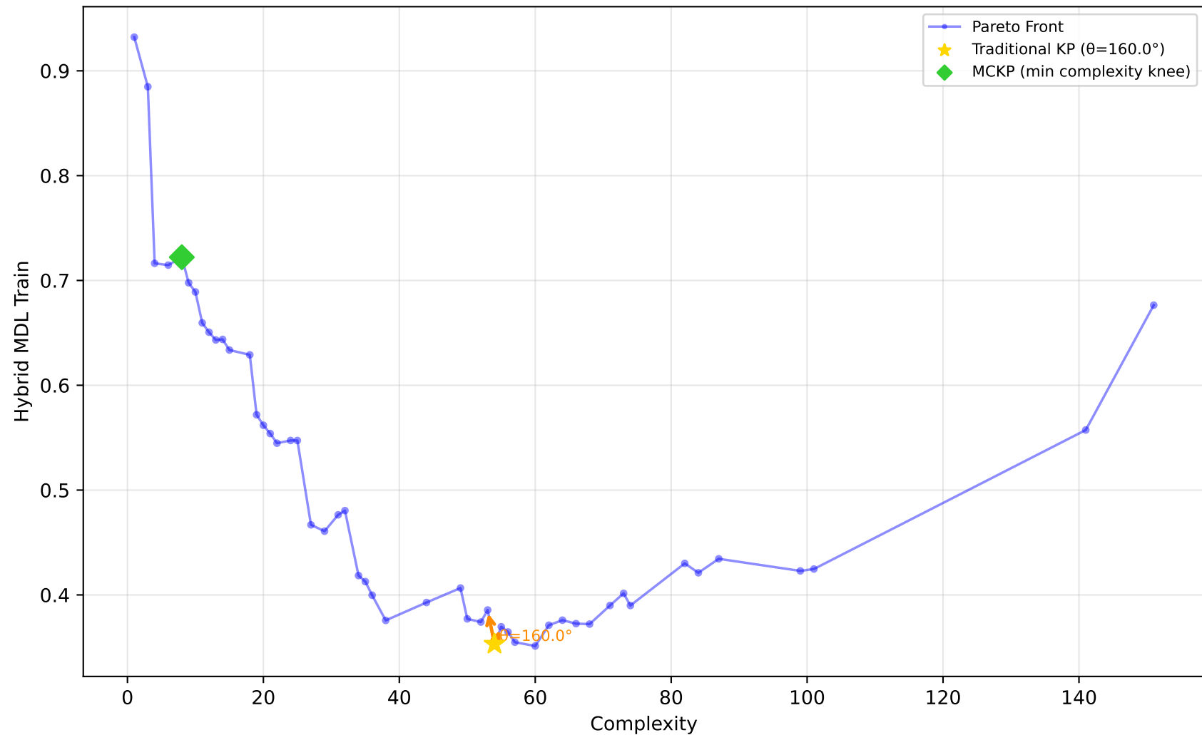
589_fri_c2_1000_25 - Run 8 - SVP - Hybrid MDL Train \lambda_1=0.10, \lambda_2=0.00, \lambda_3=0.10 | Difficulty: 1.00 | Method: hmr
