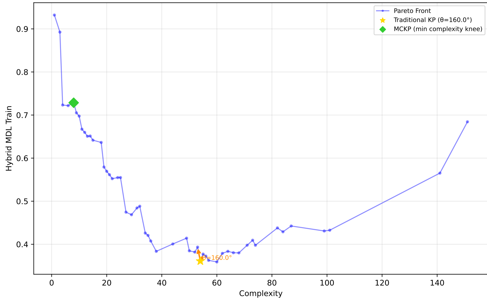
589_fri_c2_1000_25 - Run 8 - SVP - Hybrid MDL Train \lambda_1=0.20, \lambda_2=0.00, \lambda_3=1.00 | Difficulty: 1.00 | Method: hmr
