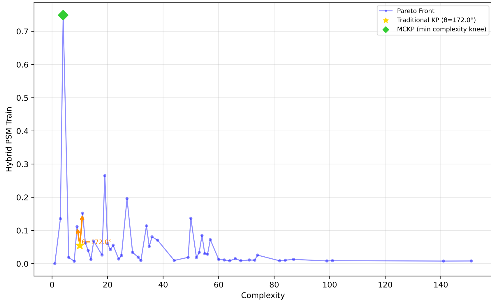
589_fri_c2_1000_25 - Run 8 - SVP - Hybrid PSM Train \lambda_1=0.10, \lambda_2=0.00, \lambda_3=0.10 | Difficulty: 1.00 | Method: hmr
