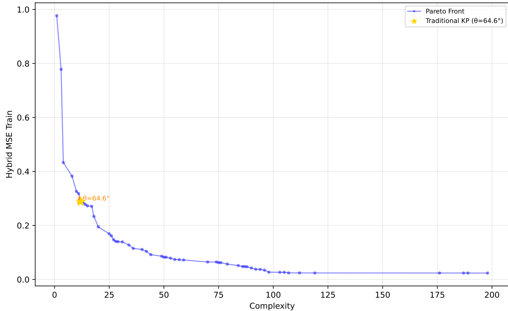
589_fri_c2_1000_25 - Run 9 - MVP - Hybrid MSE Train \lambda_1=0.00, \bar{\lambda}_2=0.00, \bar{\lambda}_3=0.00 | Difficulty: 1.00 | Method: hmr
