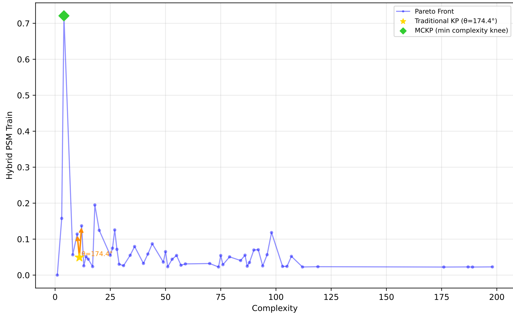
589_fri_c2_1000_25 - Run 9 - MVP - Hybrid PSM Train \lambda_1=0.30, \bar{\lambda}_2=0.00, \bar{\lambda}_3=0.20 | Difficulty: 1.00 | Method: hmr
