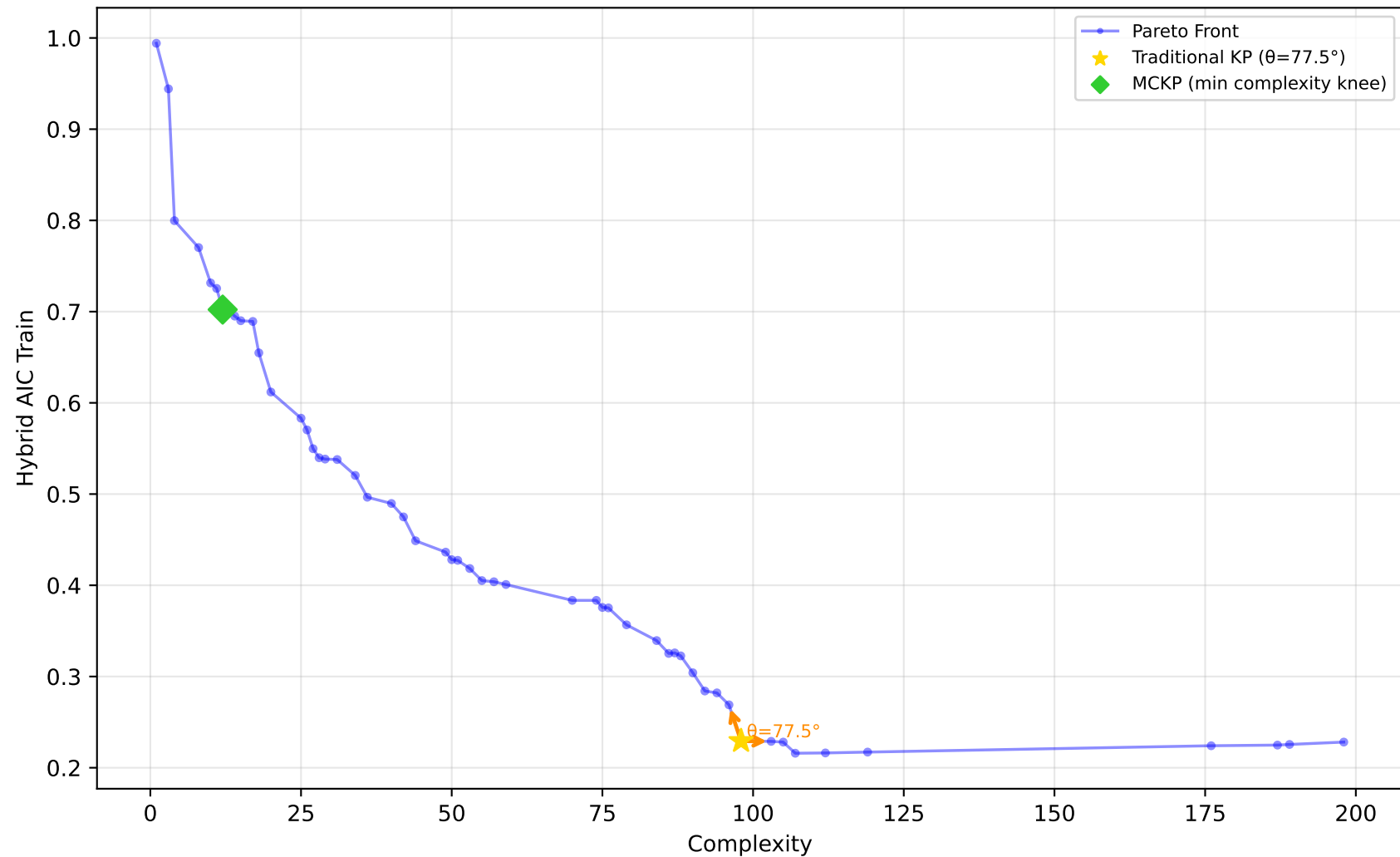
589_fri_c2_1000_25 - Run 9 - SVP - Hybrid AIC Train \lambda_1=0.10, \lambda_2=0.00, \lambda_3=0.10 | Difficulty: 1.00 | Method: hmr
