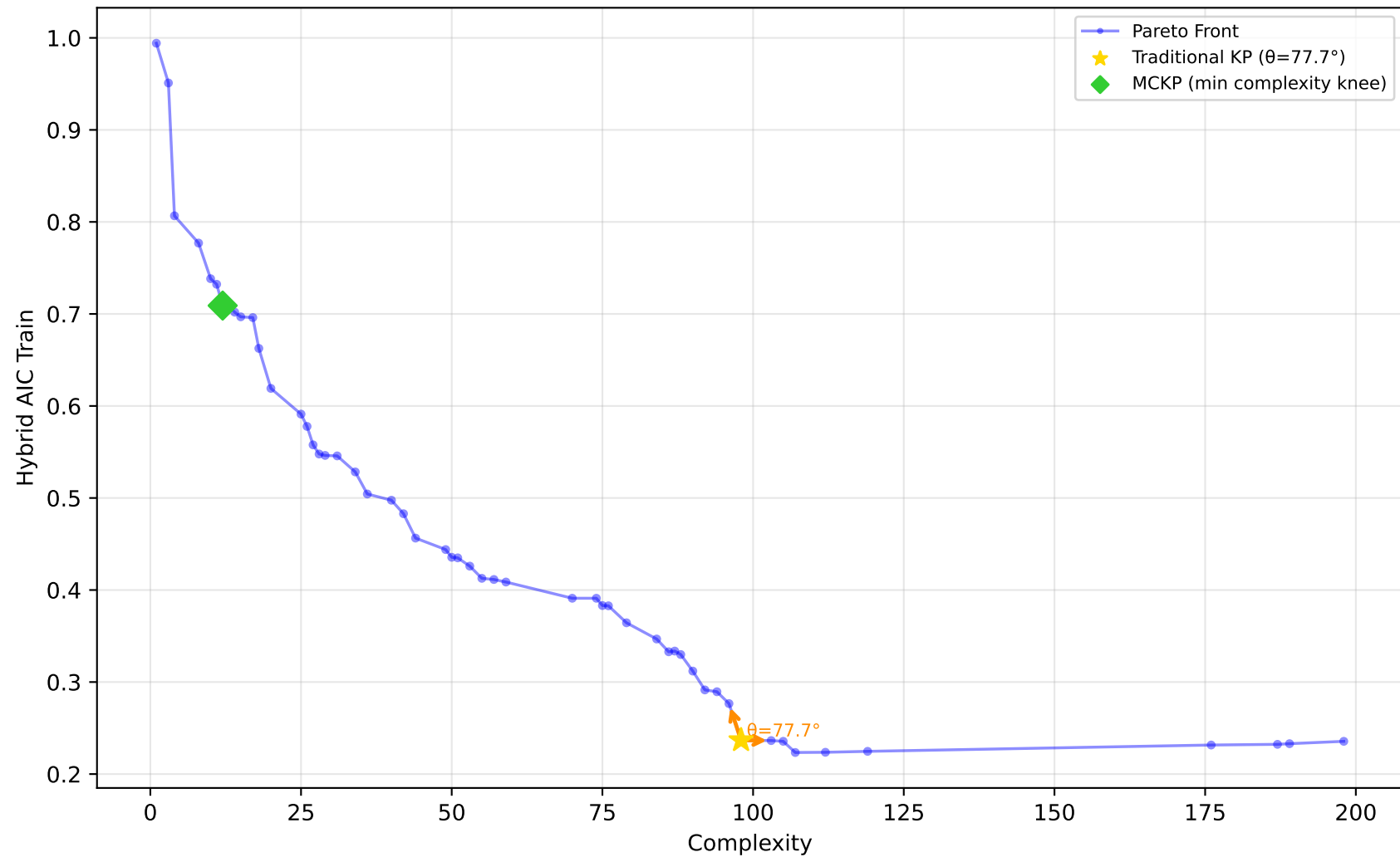
589_fri_c2_1000_25 - Run 9 - SVP - Hybrid AIC Train \lambda_1=0.20, \lambda_2=0.00, \lambda_3=1.00 | Difficulty: 1.00 | Method: hmr
