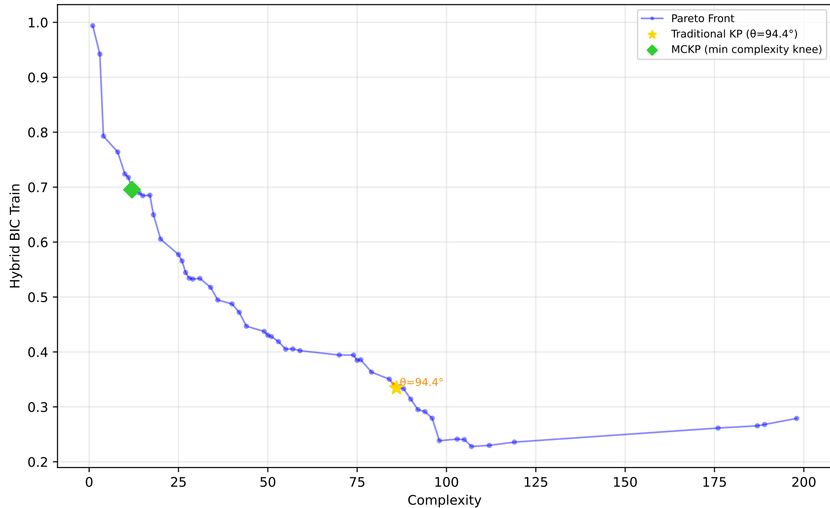
589_fri_c2_1000_25 - Run 9 - SVP - Hybrid BIC Train \lambda_1=0.10, \lambda_2=0.00, \lambda_3=0.10 | Difficulty: 1.00 | Method: hmr
