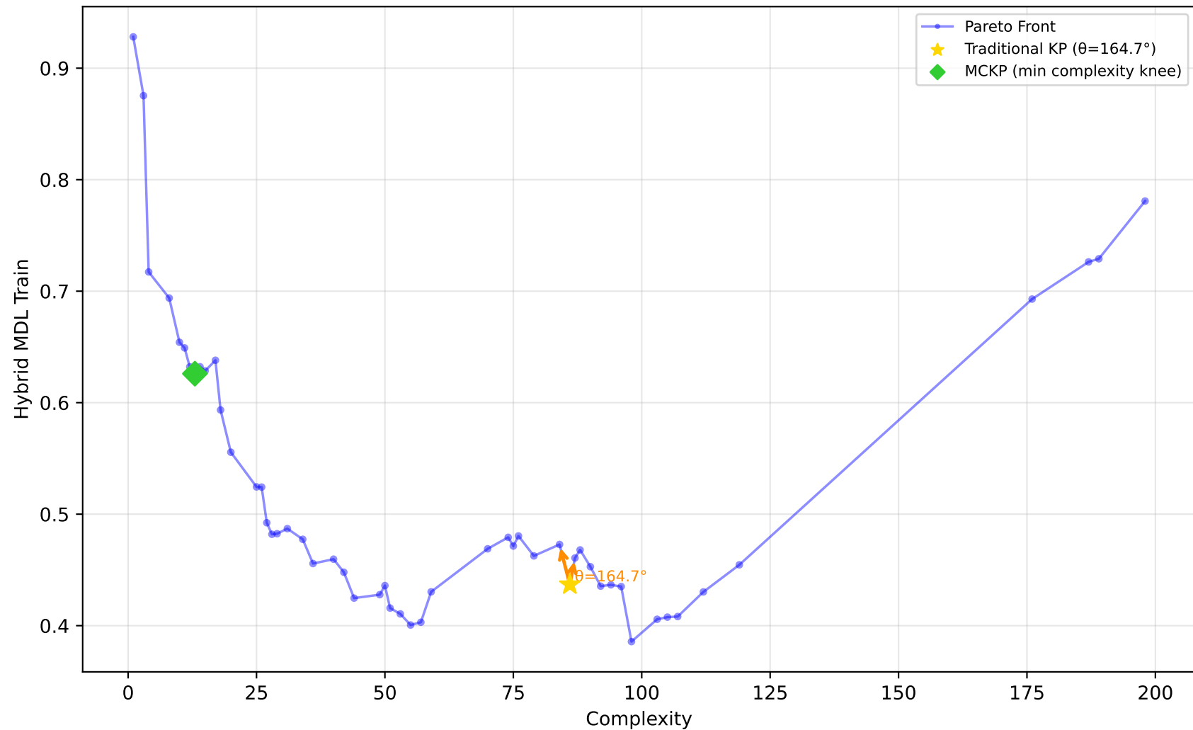
589_fri_c2_1000_25 - Run 9 - SVP - Hybrid MDL Train \lambda_1=0.10, \lambda_2=0.00, \lambda_3=0.10 | Difficulty: 1.00 | Method: hmr
