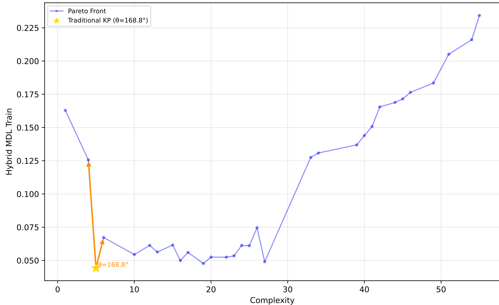
1028_SWD - Run 10 - MVP - Hybrid MDL Train \lambda_1=0.00, \lambda_2=0.00, \lambda_3=0.00 | Difficulty: 1.00 | Method: hmr
