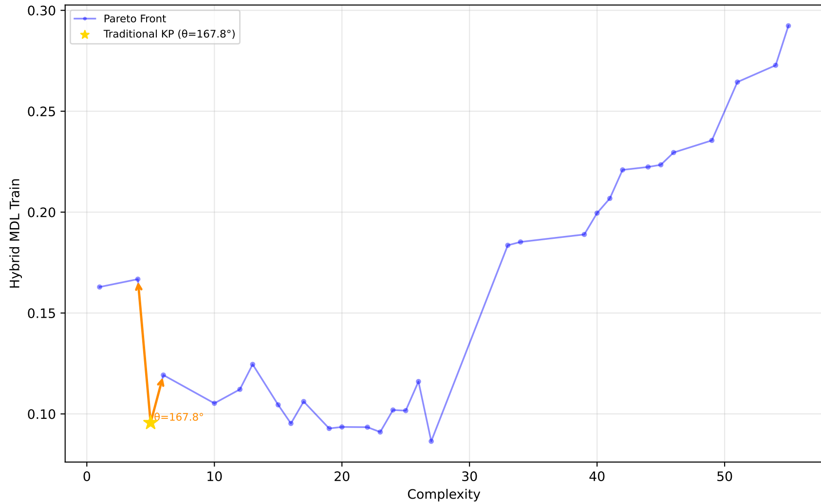
1028_SWD - Run 10 - MVP - Hybrid MDL Train \lambda_1=0.60, \lambda_2=0.00, \lambda_3=0.00 | Difficulty: 1.00 | Method: hmr
