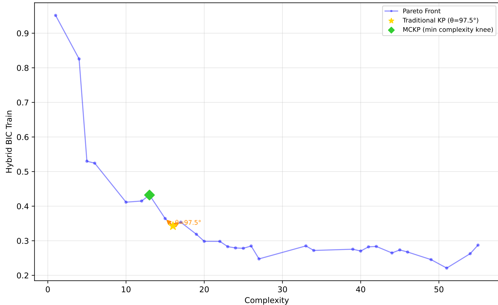
1028_SWD - Run 10 - SVP - Hybrid BIC Train \lambda_1=0.60, \lambda_2=0.00, \lambda_3=0.00 | Difficulty: 1.00 | Method: hmr
