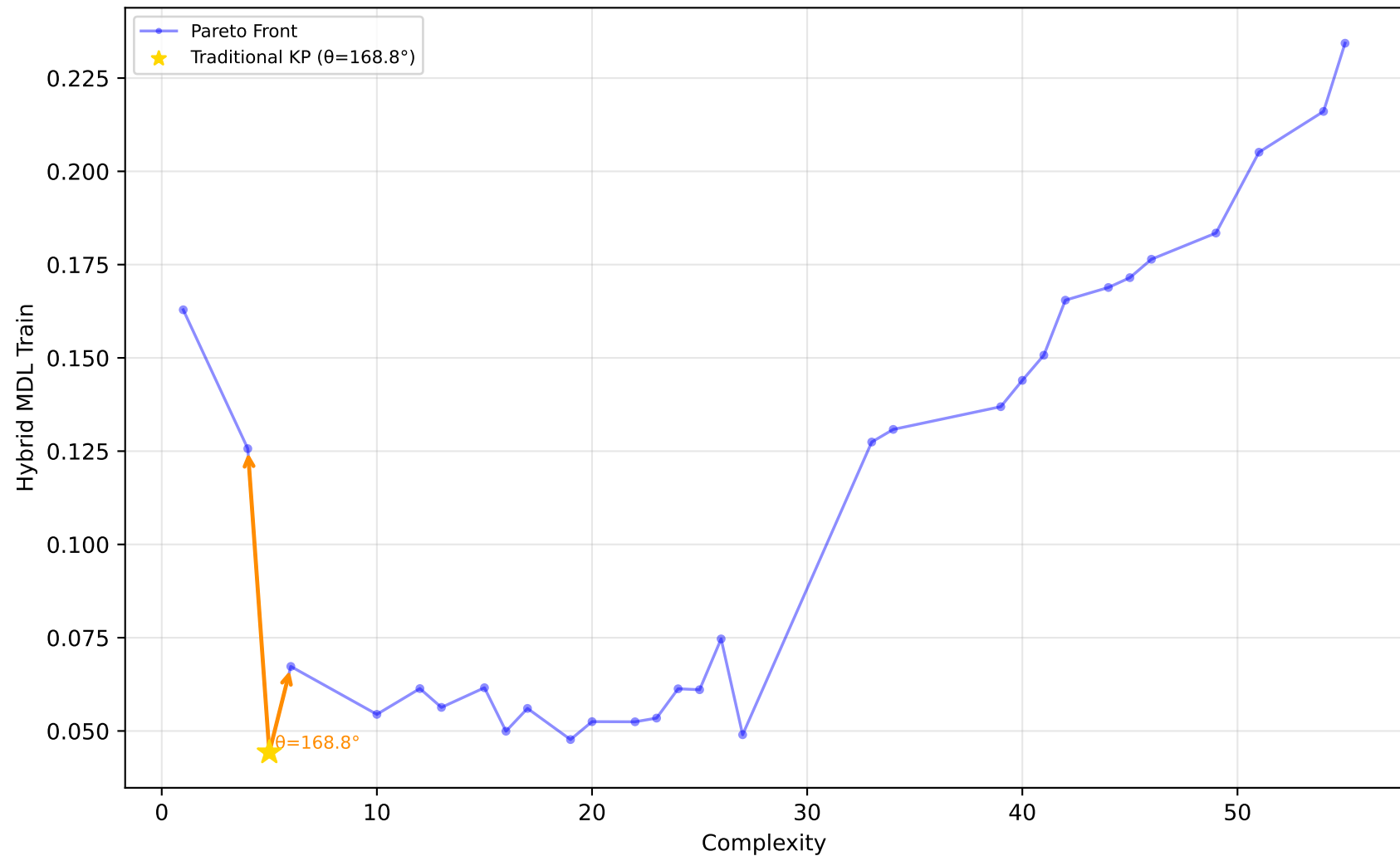
1028_SWD - Run 10 - SVP - Hybrid MDL Train \lambda_1=0.00, \lambda_2=0.60, \lambda_3=0.00 | Difficulty: 1.00 | Method: hmr
