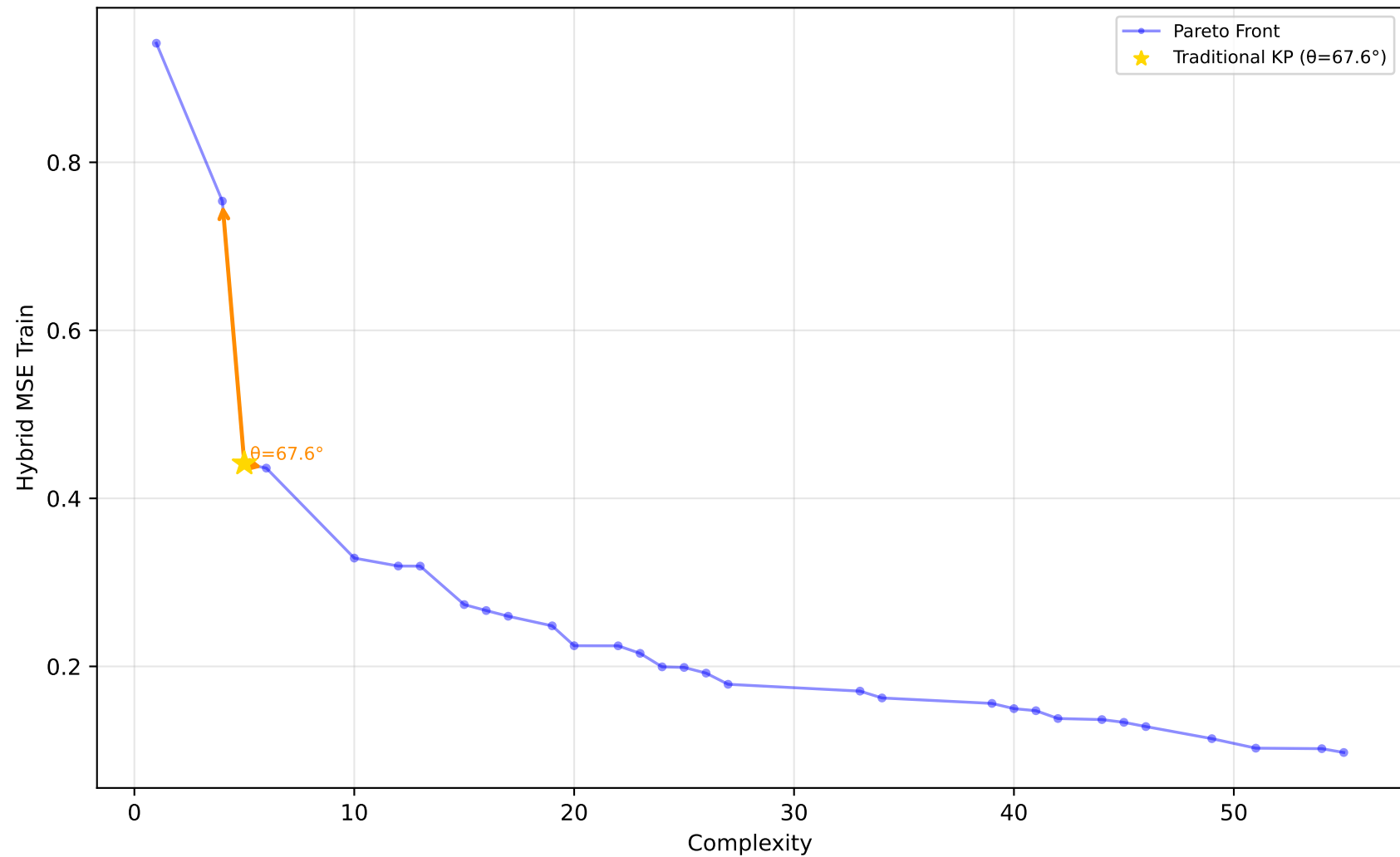
1028_SWD - Run 10 - SVP - Hybrid MSE Train \lambda_1=0.00, \lambda_2=0.60, \lambda_3=0.00 | Difficulty: 1.00 | Method: hmr
