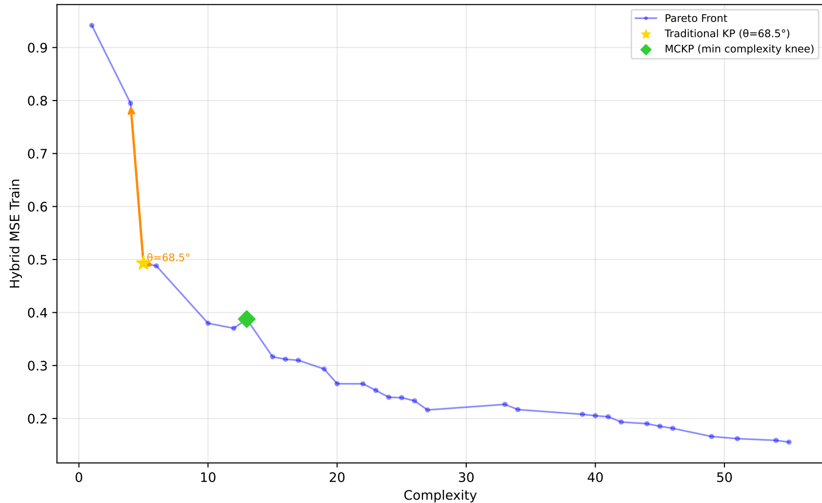
1028_SWD - Run 10 - SVP - Hybrid MSE Train \lambda_1=0.60, \lambda_2=0.00, \lambda_3=0.00 | Difficulty: 1.00 | Method: hmr
