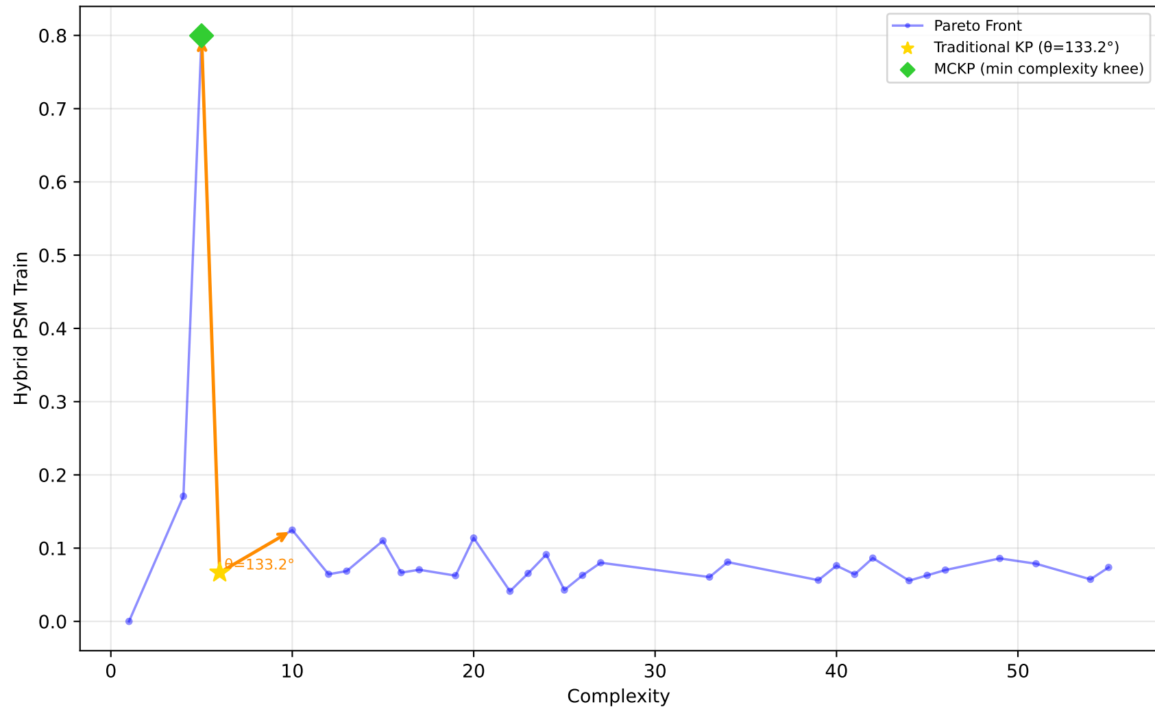
1028_SWD - Run 10 - SVP - Hybrid PSM Train \lambda_1=0.60, \lambda_2=0.00, \lambda_3=0.00 | Difficulty: 1.00 | Method: hmr
