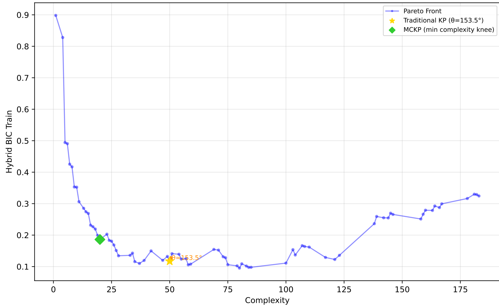
1028_SW D - Run 11 - MVP - Hybrid BIC Train \lambda_1=0.60, \lambda_2=0.00, \lambda_3=0.00 | Difficulty: 1.00 | Method: hmr
