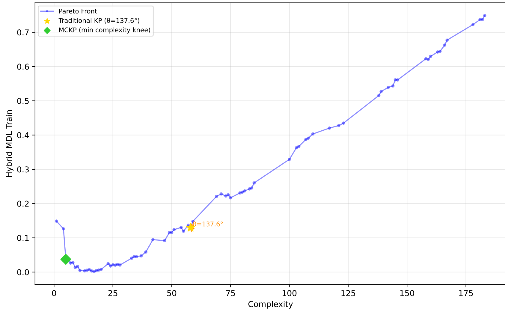
1028_SWD - Run 11 - MVP - Hybrid MDL Train \lambda_1=0.00, \lambda_2=0.00, \lambda_3=0.00 | Difficulty: 1.00 | Method: hmr
