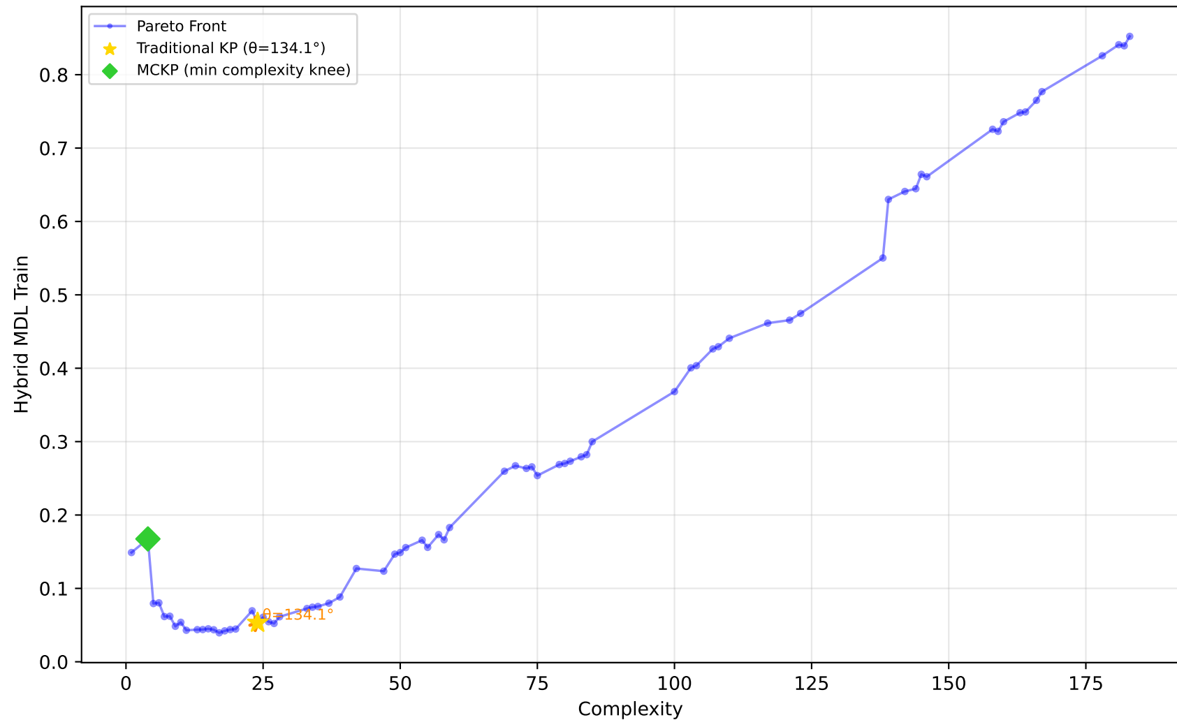
1028_SWD - Run 11 - MVP - Hybrid MDL Train \lambda_1=0.60, \lambda_2=0.00, \lambda_3=0.00 | Difficulty: 1.00 | Method: hmr
