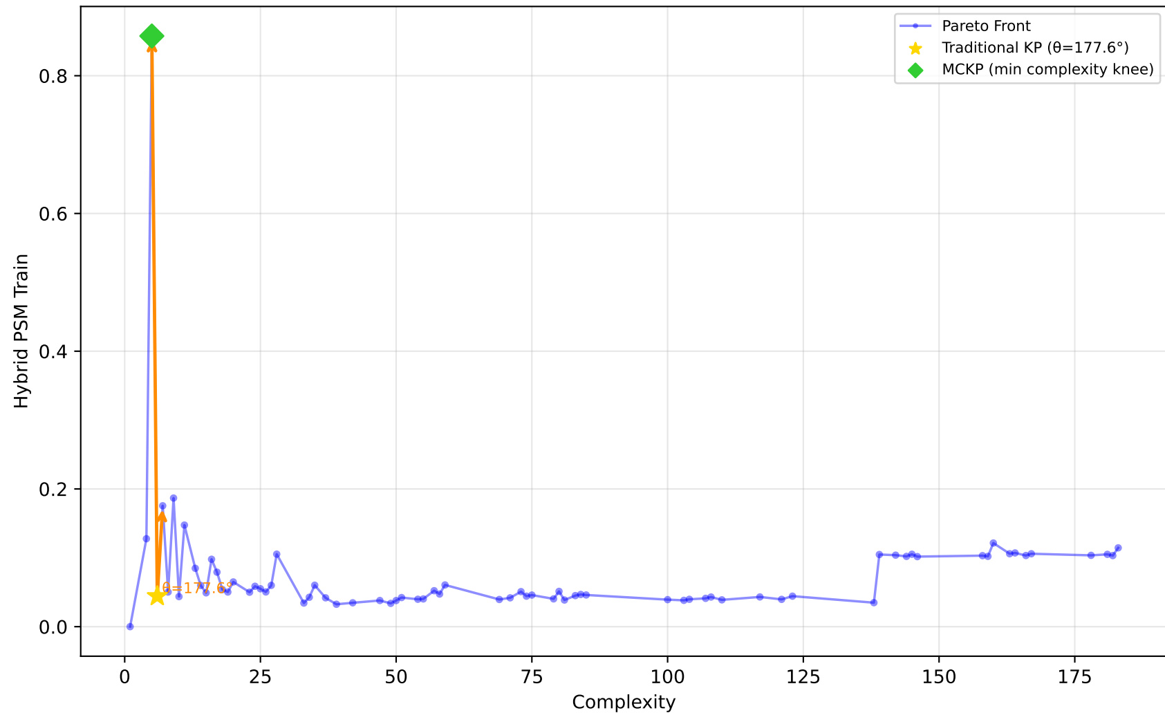
1028_SWD - Run 11 - MVP - Hybrid PSM Train \lambda_1=0.60, \lambda_2=0.00, \lambda_3=0.00 | Difficulty: 1.00 | Method: hmr
