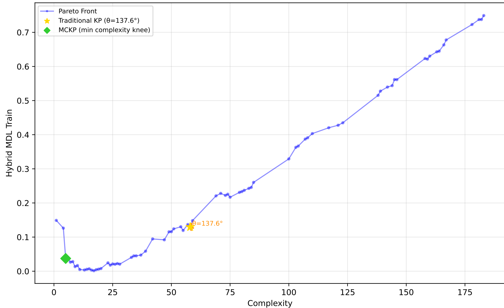
1028_SWD - Run 11 - SVP - Hybrid MDL Train \lambda_1=0.00, \lambda_2=0.60, \lambda_3=0.00 | Difficulty: 1.00 | Method: hmr
