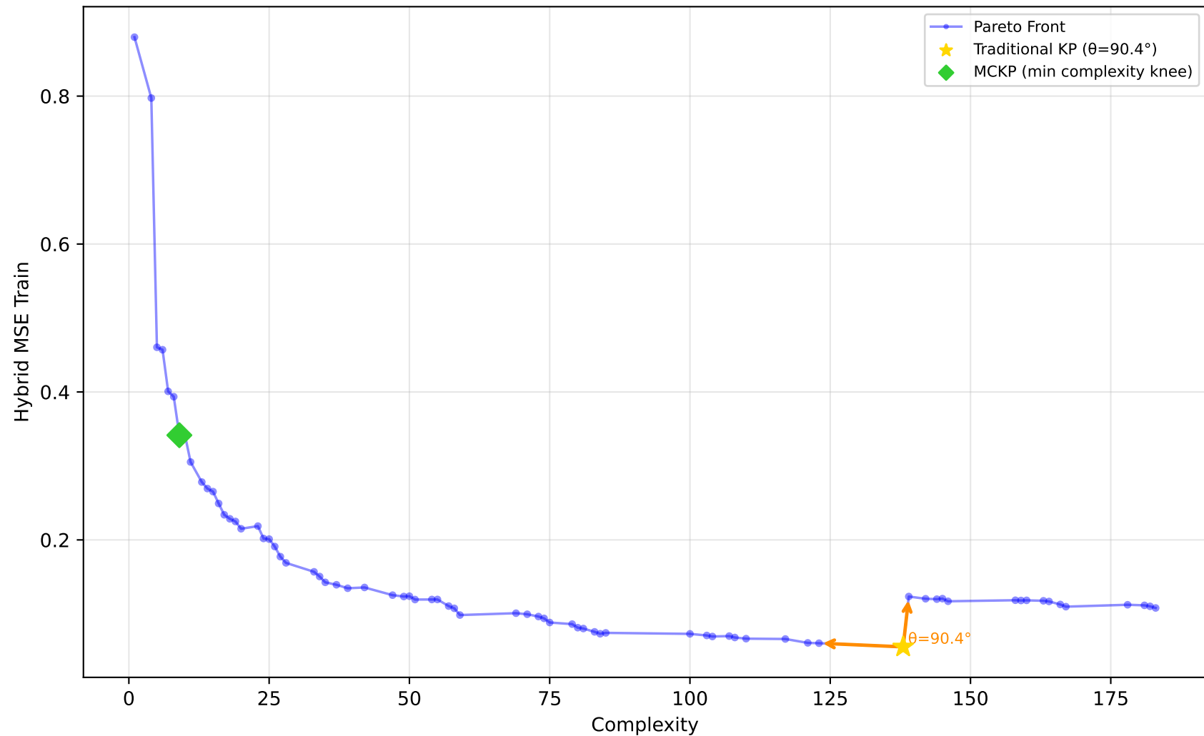
1028_SWD - Run 11 - SVP - Hybrid MSE Train \lambda_1=0.60, \lambda_2=0.00, \lambda_3=0.00 | Difficulty: 1.00 | Method: hmr
