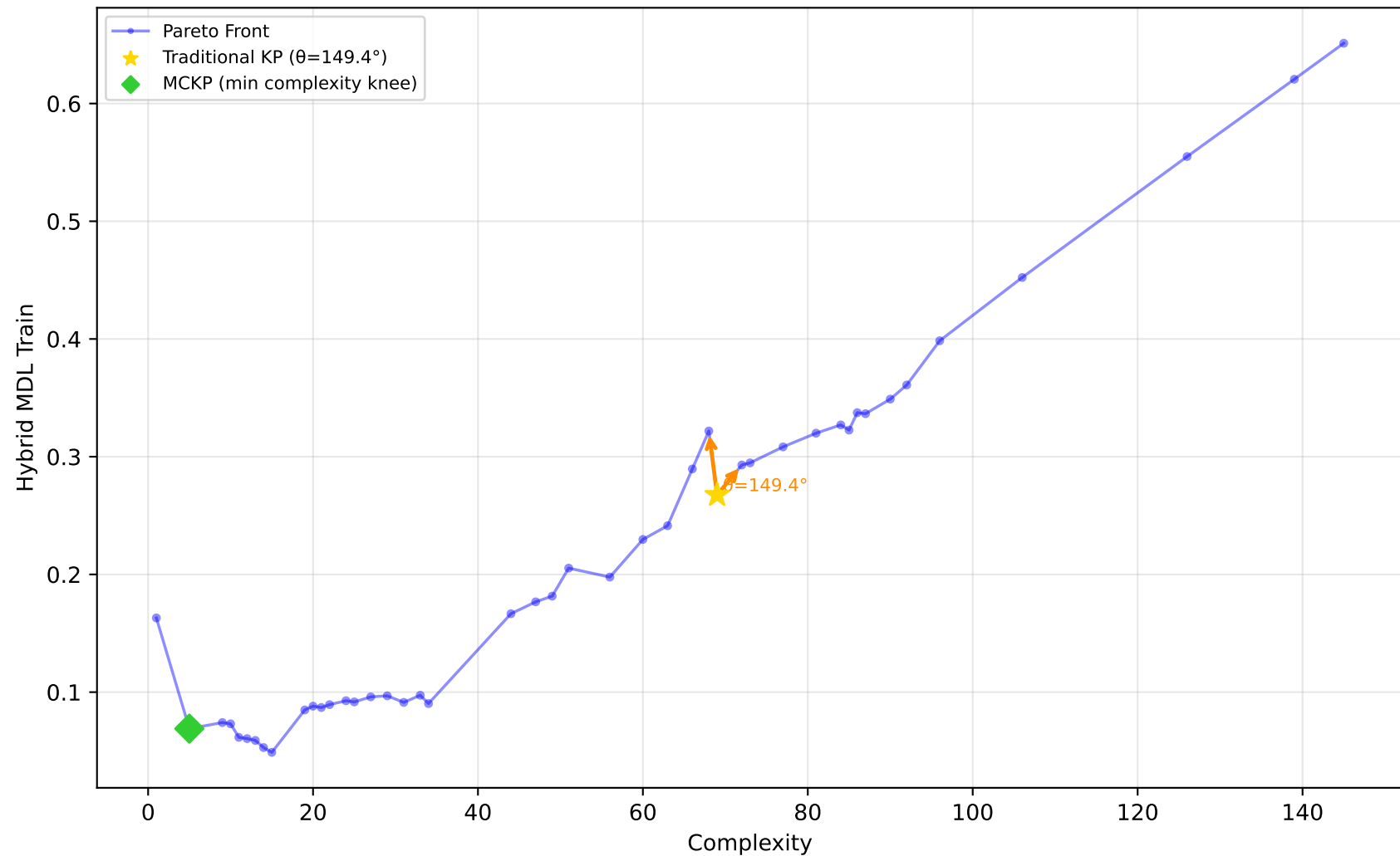
1028_SWD - Run 12 - MVP - Hybrid MDL Train \lambda_1=0.00, \lambda_2=0.00, \lambda_3=0.00 | Difficulty: 1.00 | Method: hmr
