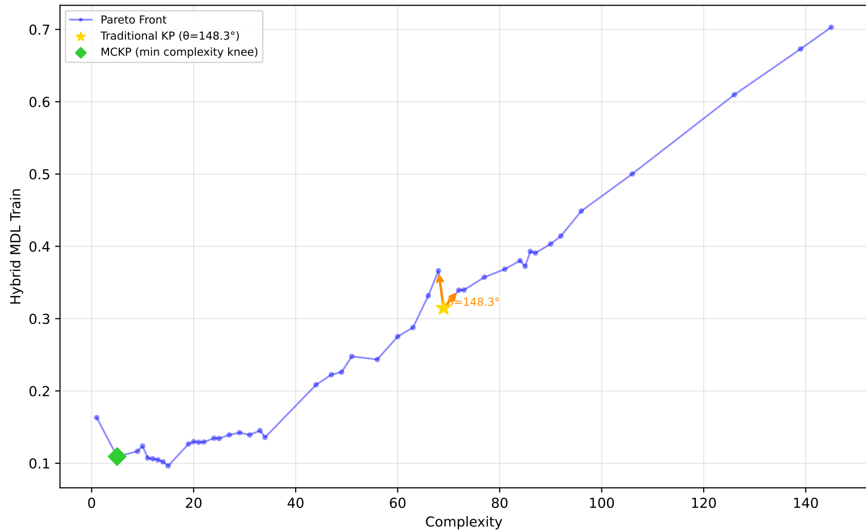
1028_SWD - Run 12 - MVP - Hybrid MDL Train \lambda_1=0.60, \lambda_2=0.00, \lambda_3=0.00 | Difficulty: 1.00 | Method: hmr
