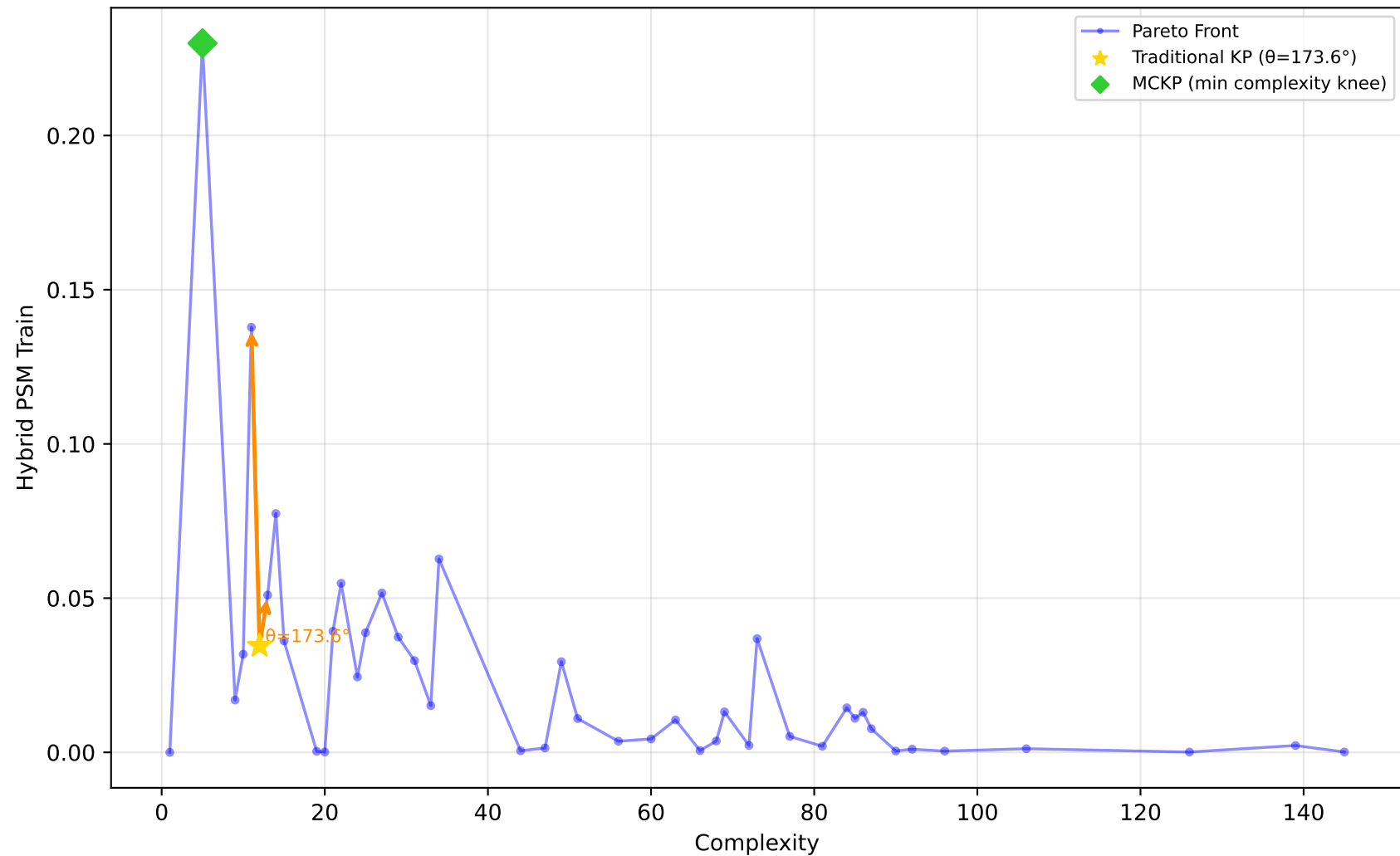
1028_SWD - Run 12 - MVP - Hybrid PSM Train \lambda_1=0.00, \lambda_2=0.00, \lambda_3=0.00 | Difficulty: 1.00 | Method: hmr
