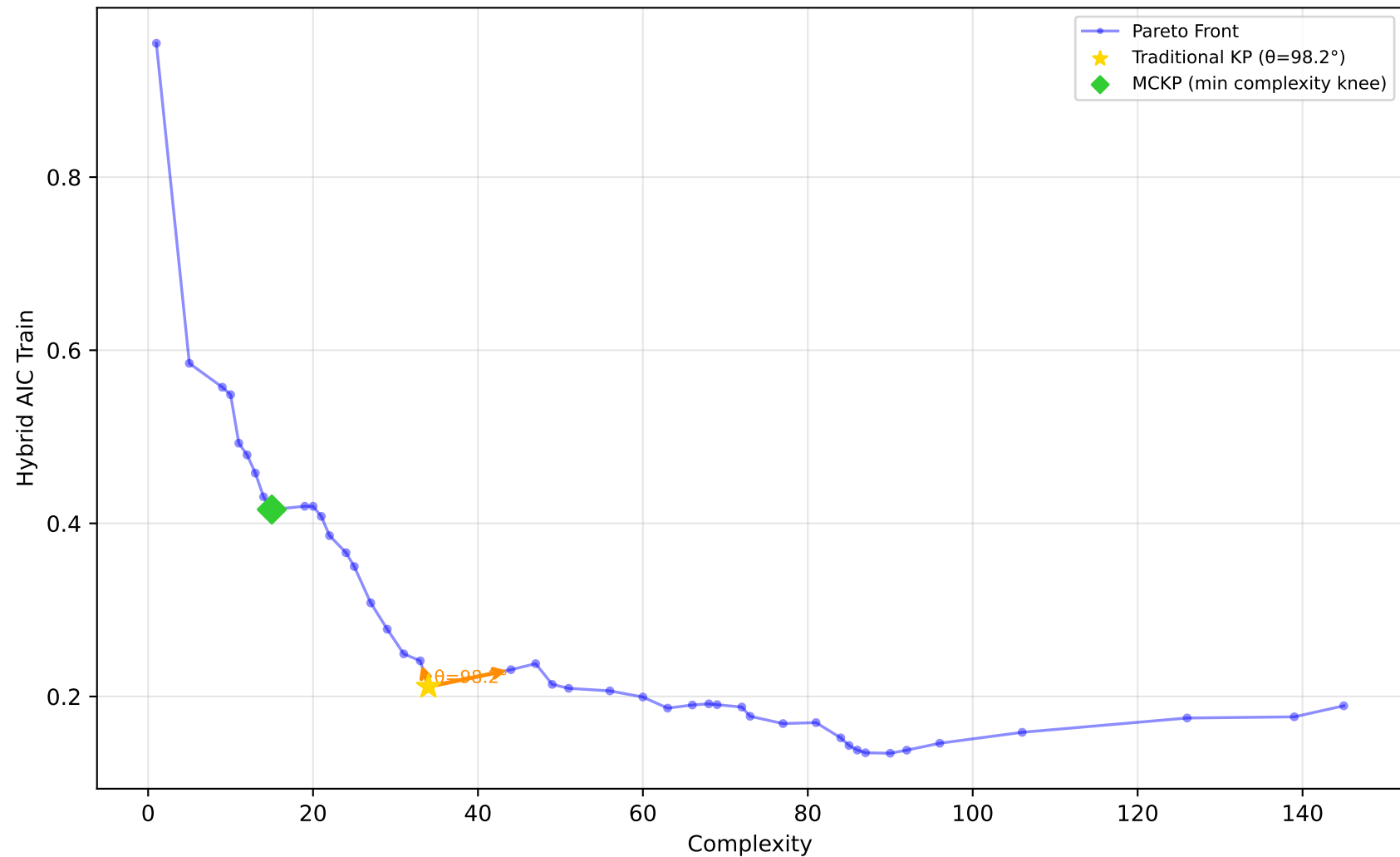
1028_SWD - Run 12 - SVP - Hybrid AIC Train \lambda_1=0.00, \lambda_2=0.60, \lambda_3=0.00 | Difficulty: 1.00 | Method: hmr
