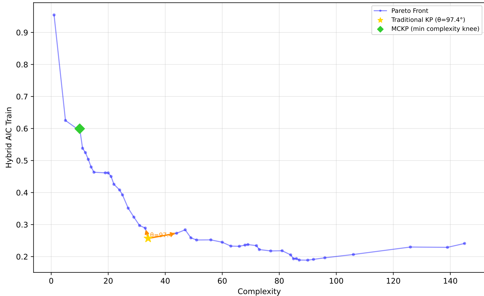
1028_SWD - Run 12 - SVP - Hybrid AIC Train \lambda_1=0.60, \lambda_2=0.00, \lambda_3=0.00 | Difficulty: 1.00 | Method: hmr
