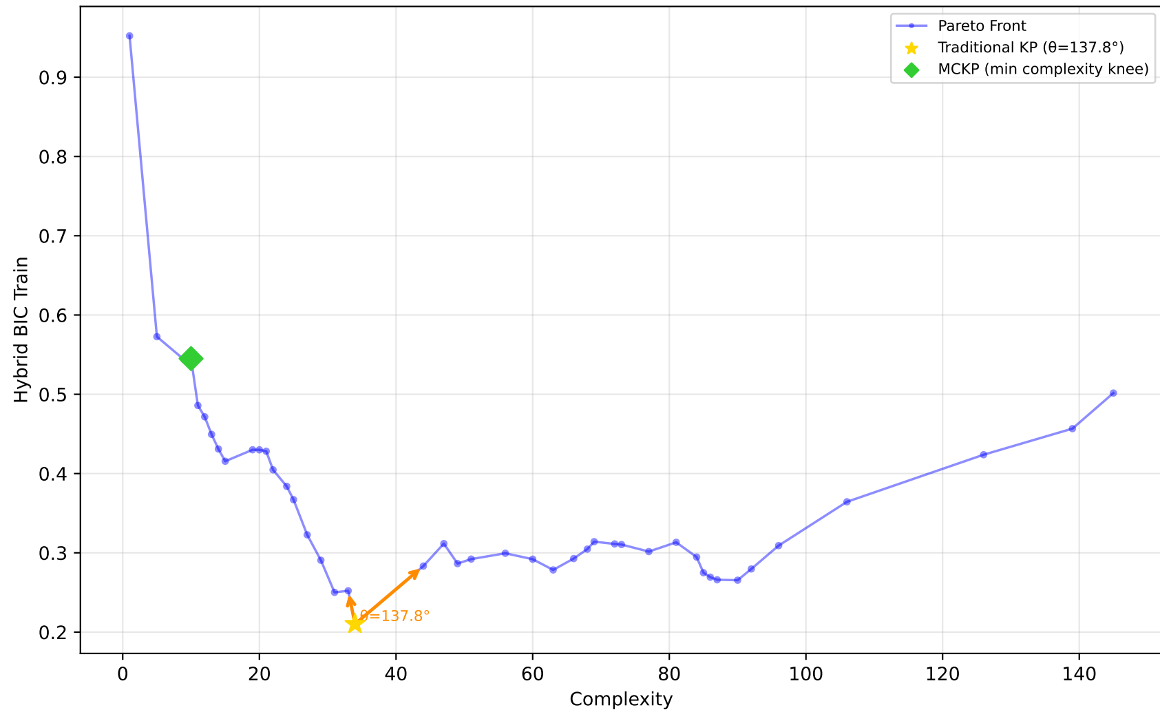
1028_SWD - Run 12 - SVP - Hybrid BIC Train \lambda_1=0.00, \lambda_2=0.60, \lambda_3=0.00 | Difficulty: 1.00 | Method: hmr
