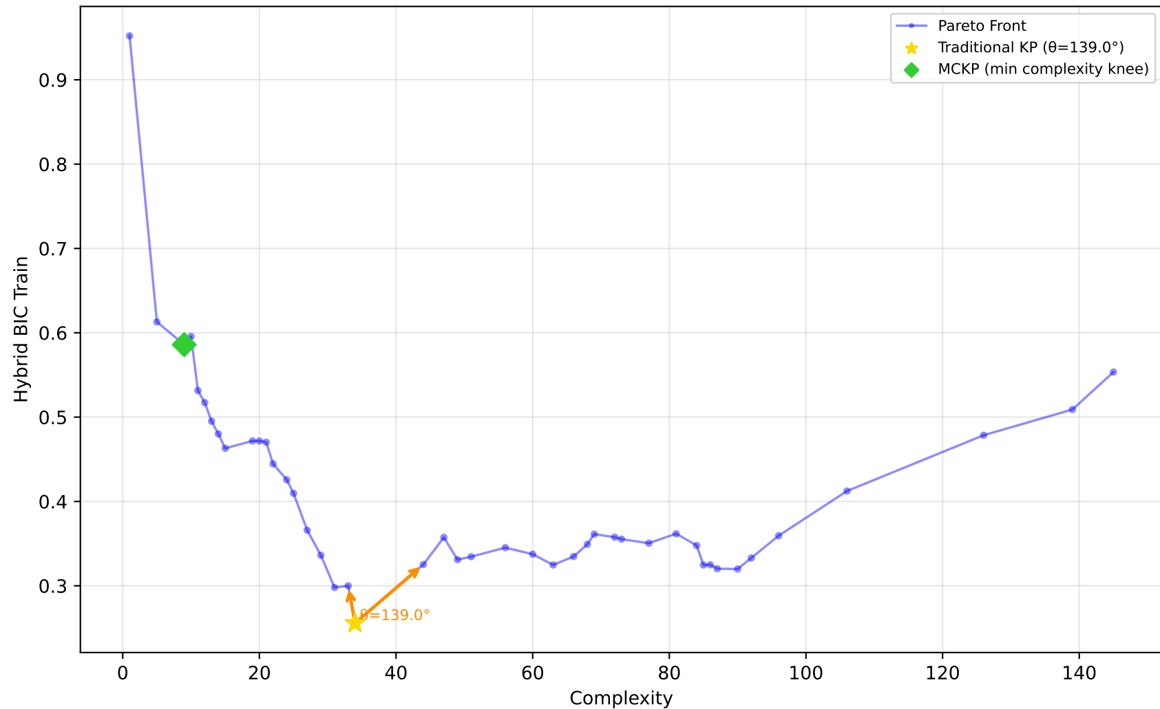
1028_SWD - Run 12 - SVP - Hybrid BIC Train \lambda_1=0.60, \lambda_2=0.00, \lambda_3=0.00 | Difficulty: 1.00 | Method: hmr
