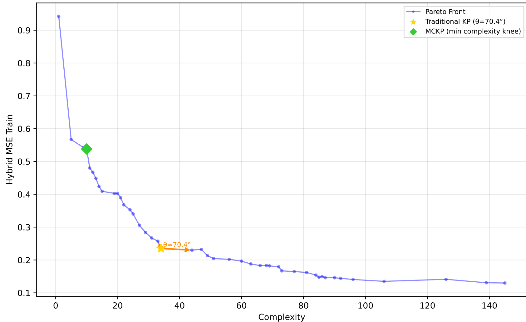
1028_SWD - Run 12 - SVP - Hybrid MSE Train \lambda_1=0.60, \lambda_2=0.00, \lambda_3=0.00 | Difficulty: 1.00 | Method: hmr
