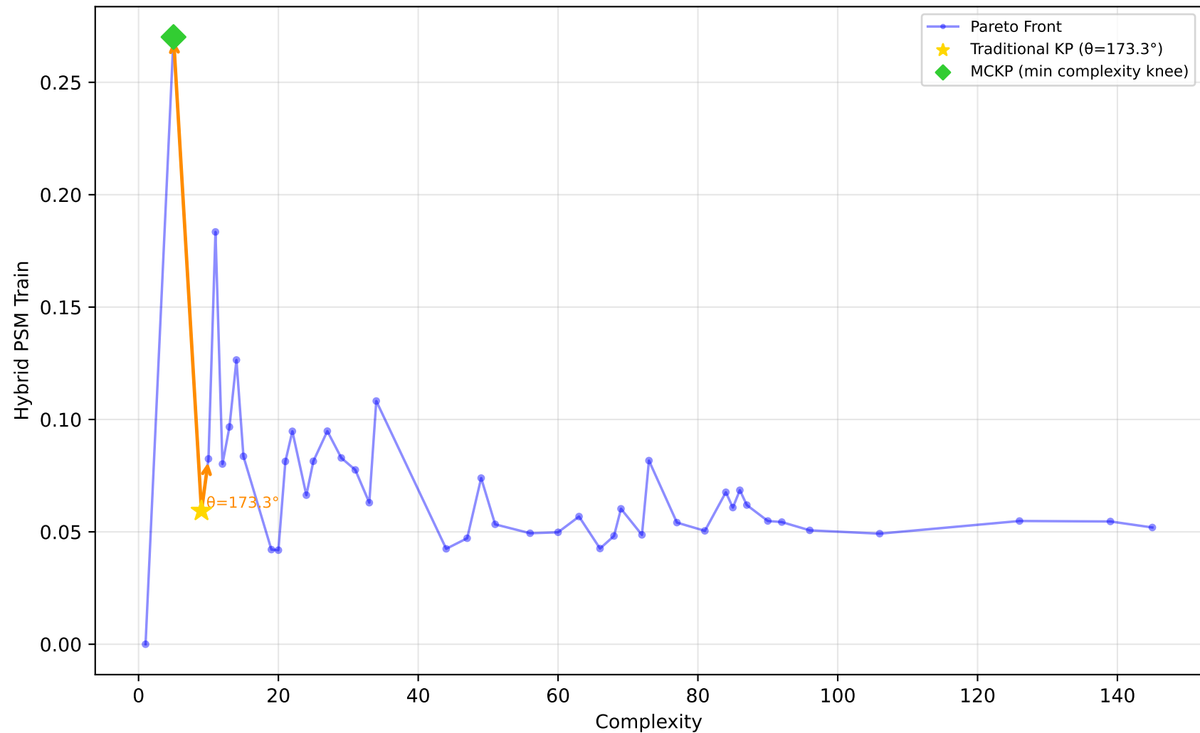
1028_SWD - Run 12 - SVP - Hybrid PSM Train \lambda_1=0.60, \lambda_2=0.00, \lambda_3=0.00 | Difficulty: 1.00 | Method: hmr
