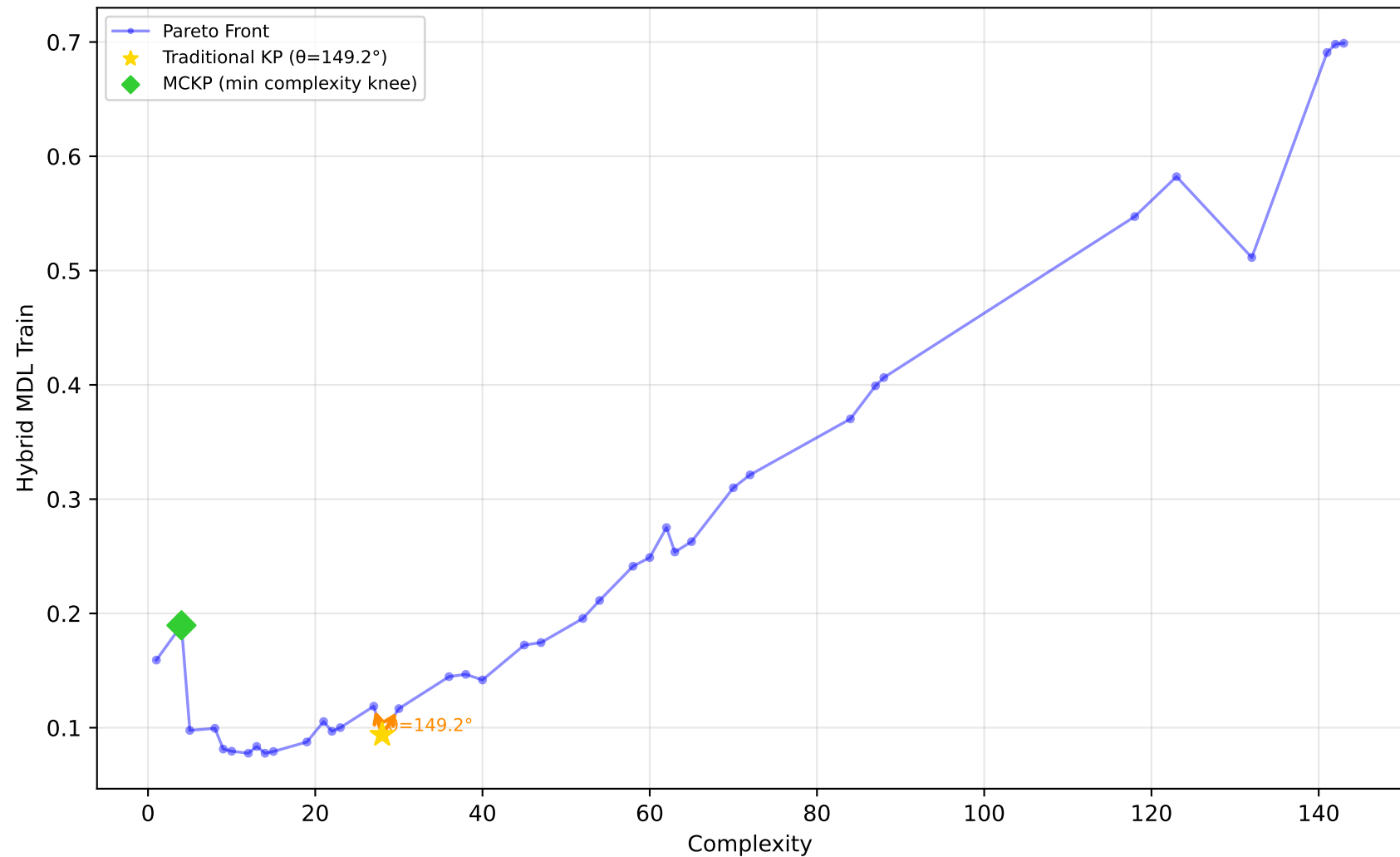
1028_SWD - Run 13 - MVP - Hybrid MDL Train \lambda_1=0.60, \lambda_2=0.00, \lambda_3=0.00 | Difficulty: 1.00 | Method: hmr
